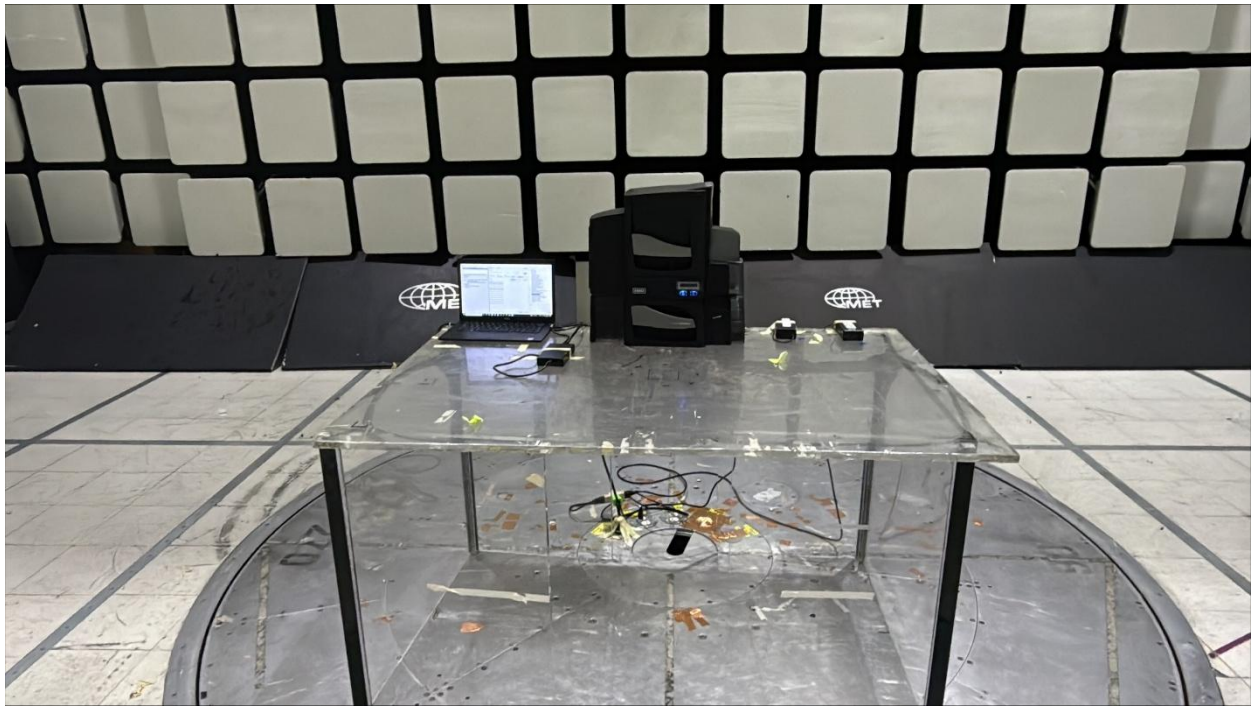
Radiated Emissions Front
