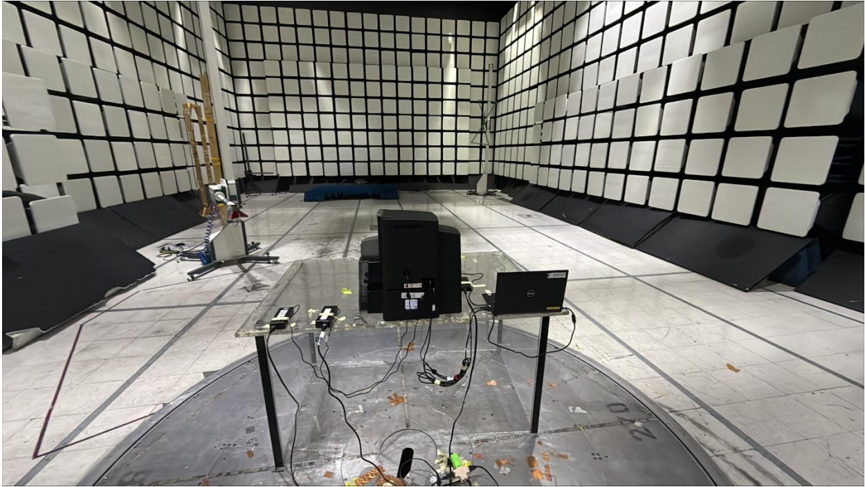
Radiated Emissions Back
