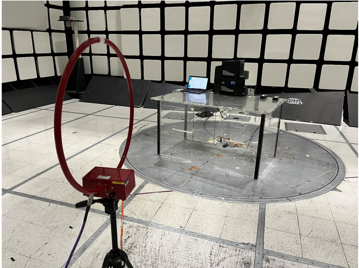
Radiated Emissions 9kHz - 30MHz Antenna View
