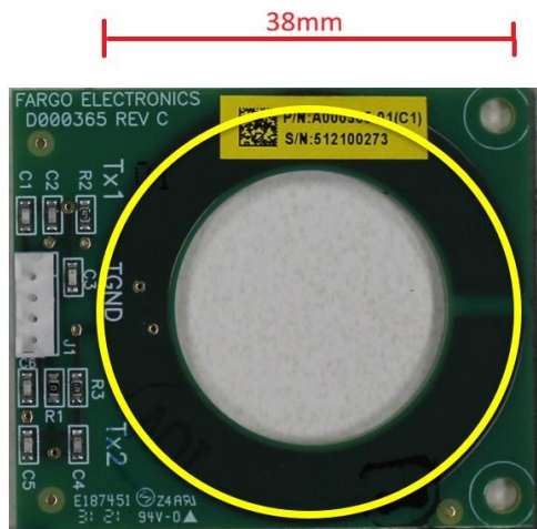
Ribbon RFID HF Antenna Dimensions
