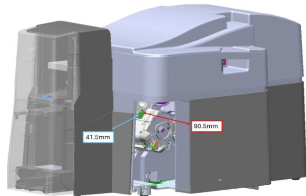
Antenna location within DTCii Plus and closest distance to outer surface of enclosure
