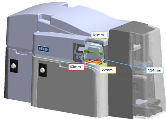
Antenna location within DTCii Plus and closest distance to outer surface of enclosure
