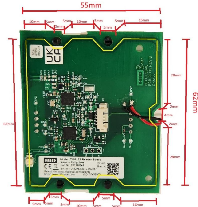
OMNIKEY 5122 HF Antenna dimensions
