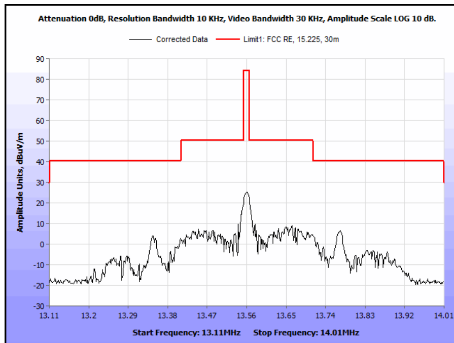
Plot 5. FCC Part 15.225 Mask, 13.110 – 14.010 MHz, 90 degree
