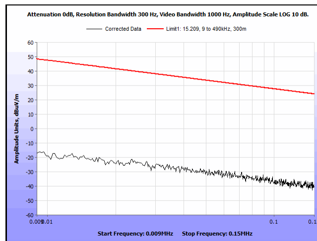
Plot 7. Spurious Emissions, Outside the Band 13.110 - 14.010 MHz, 9 – 150 kHz, 90 degrees
