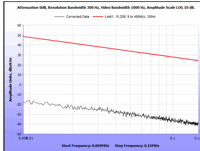
Plot 6. Spurious Emissions, Outside the Band 13.110 - 14.010 MHz, 9 – 150 kHz, 0 degrees
