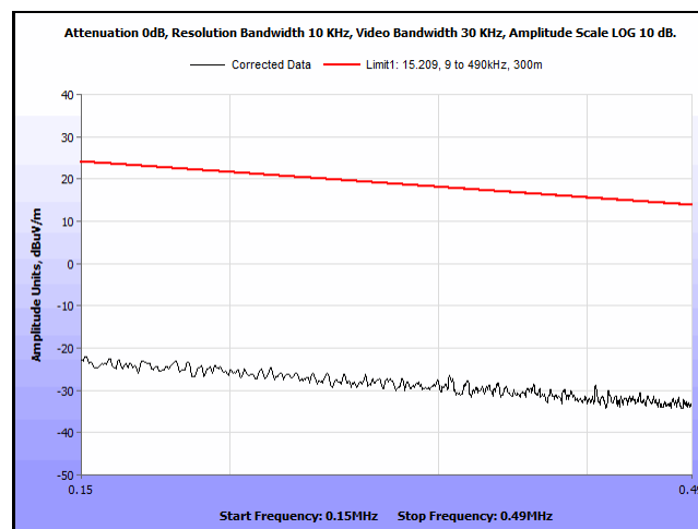
Plot 8. Spurious Emissions, Outside the Band 13.110 - 14.010 MHz, 150 – 490 kHz, 0 degrees
