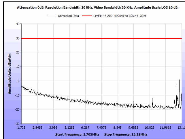
Plot 12. Spurious Emissions, Outside the Band 13.110 - 14.010 MHz, 1.705 – 13.11 MHz, 0 degrees
