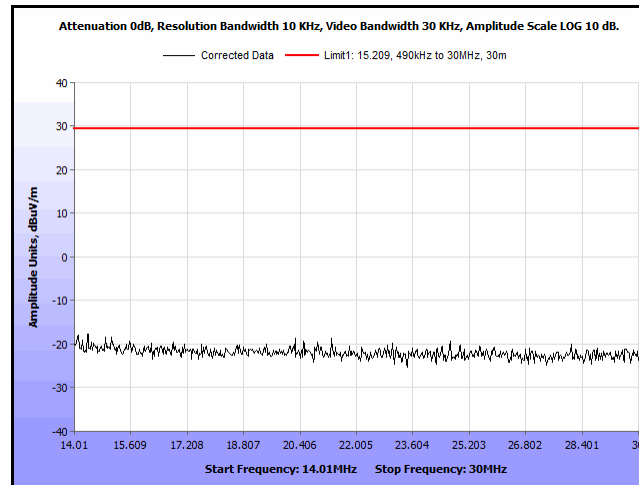
Plot 15. Spurious Emissions, Outside the Band 13.110 - 14.010 MHz, 14.010 – 30 MHz, 90 degrees
