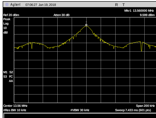
Plot 18. Frequency Stability, Vnom, 20 degrees
