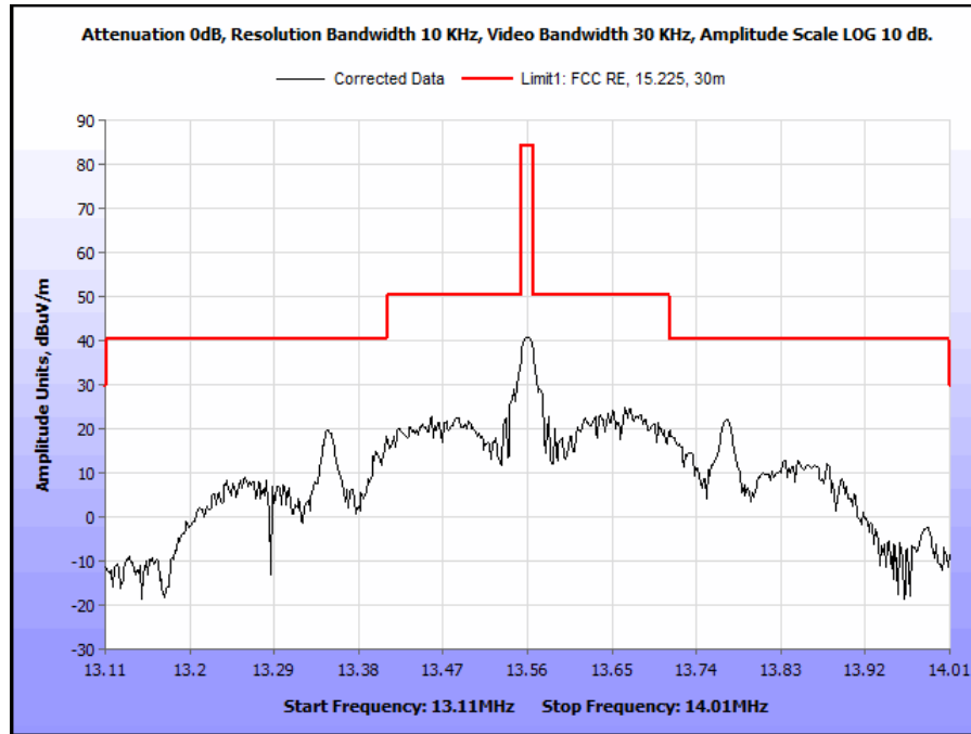
Plot 4. FCC Part 15.225 Mask, 13.110 – 14.010 MHz, 0 degree
