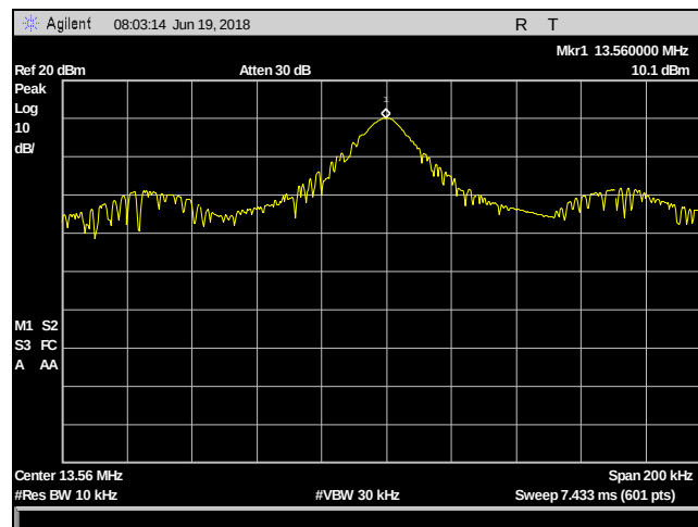
Plot 20. Frequency Stability, Vnom, 50 degrees
