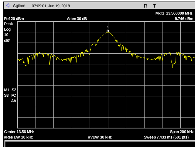
Plot 21. Frequency Stability, +15 pct, 20 degrees
