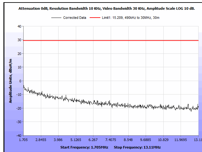
Plot 13. Spurious Emissions, Outside the Band 13.110 - 14.010 MHz, 1.705 – 13.11 MHz, 90 degrees
