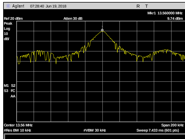
Plot 19. Frequency Stability, Vnom, -20 degrees
