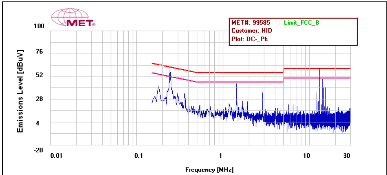
Plot 2. Conducted Emissions, DC-
