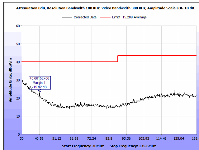
Plot 16. Spurious Emissions, Outside the Band 13.110 - 14.010 MHz, 30 – 135.6 MHz, Operating, Horizontal
