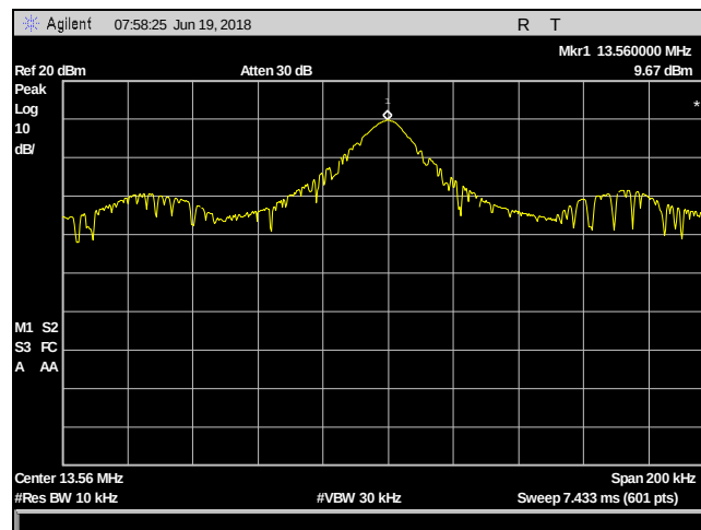
Plot 26. Frequency Stability, -15 pct, 50 degrees
