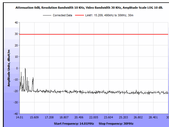
Plot 14. Spurious Emissions, Outside the Band 13.110 - 14.010 MHz, 14.010 – 30 MHz, 0 degrees
