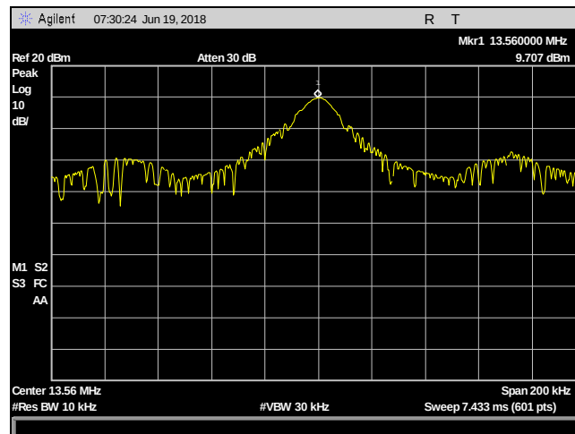
Plot 22. Frequency Stability, +15 pct, -20 degrees
