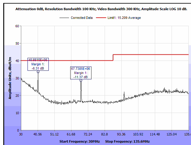
Plot 17. Spurious Emissions, Outside the Band 13.110 - 14.010 MHz, 30 – 135.6 MHz, Operating, Vertical
