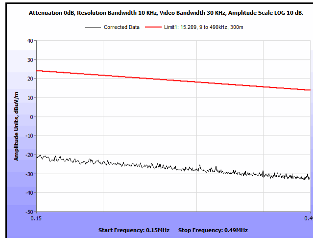
Plot 9. Spurious Emissions, Outside the Band 13.110 - 14.010 MHz, 150 – 490 kHz, 90 degrees
