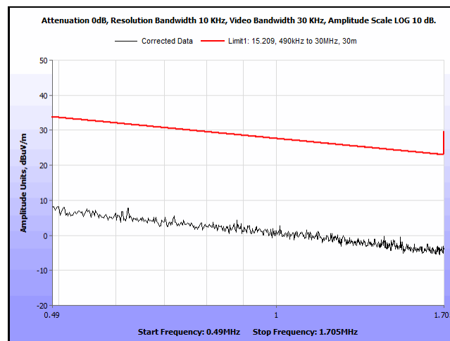
Plot 11. Spurious Emissions, Outside the Band 13.110 - 14.010 MHz, 490 kHz – 1.705 MHz, 90 degrees
