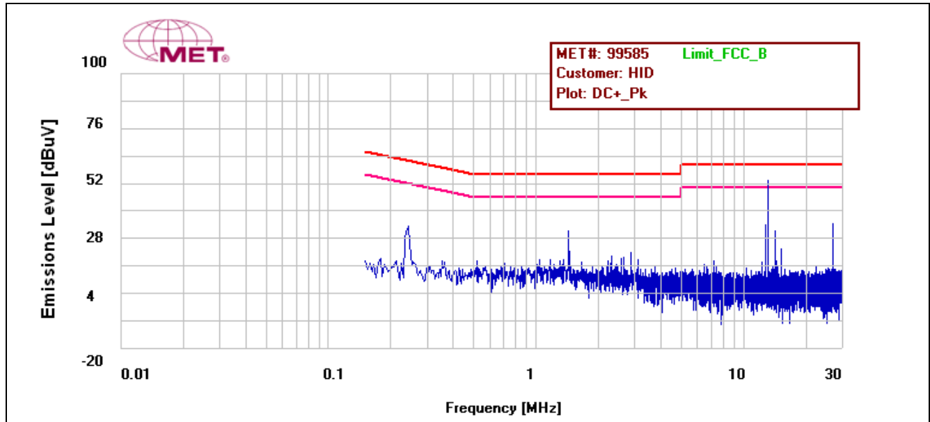
Plot 1. Conducted Emissions, DC+
