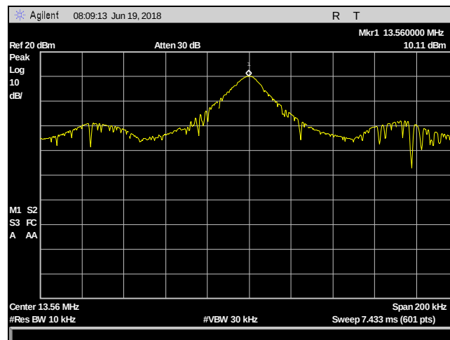
Plot 23. Frequency Stability, +15 pct, 50 degrees
