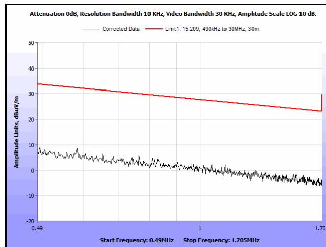
Plot 10. Spurious Emissions, Outside the Band 13.110 - 14.010 MHz, 490 kHz – 1.705 MHz, 0 degrees
