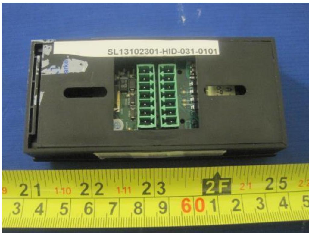
Rear View – Terminal Connector
