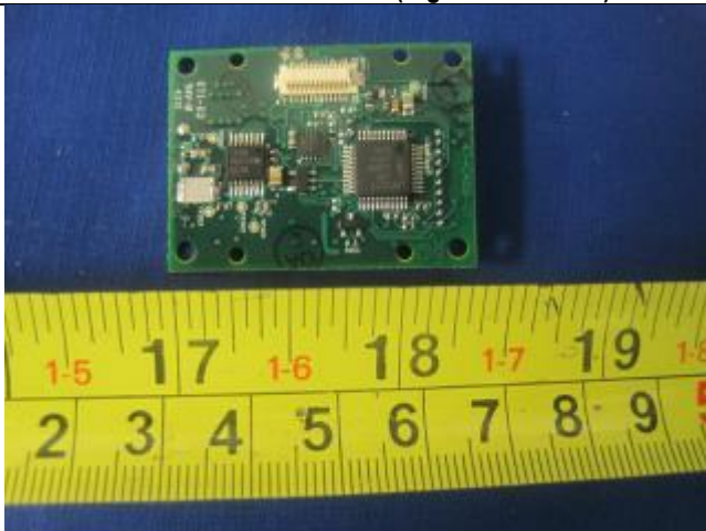
Sub PCBA Bottom View (Pigtail Connector)
