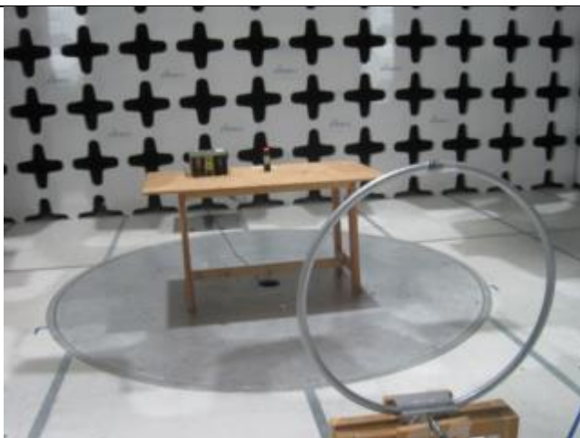
Radiated Emissions (<30MHz) – Front View (Terminal Connector)
