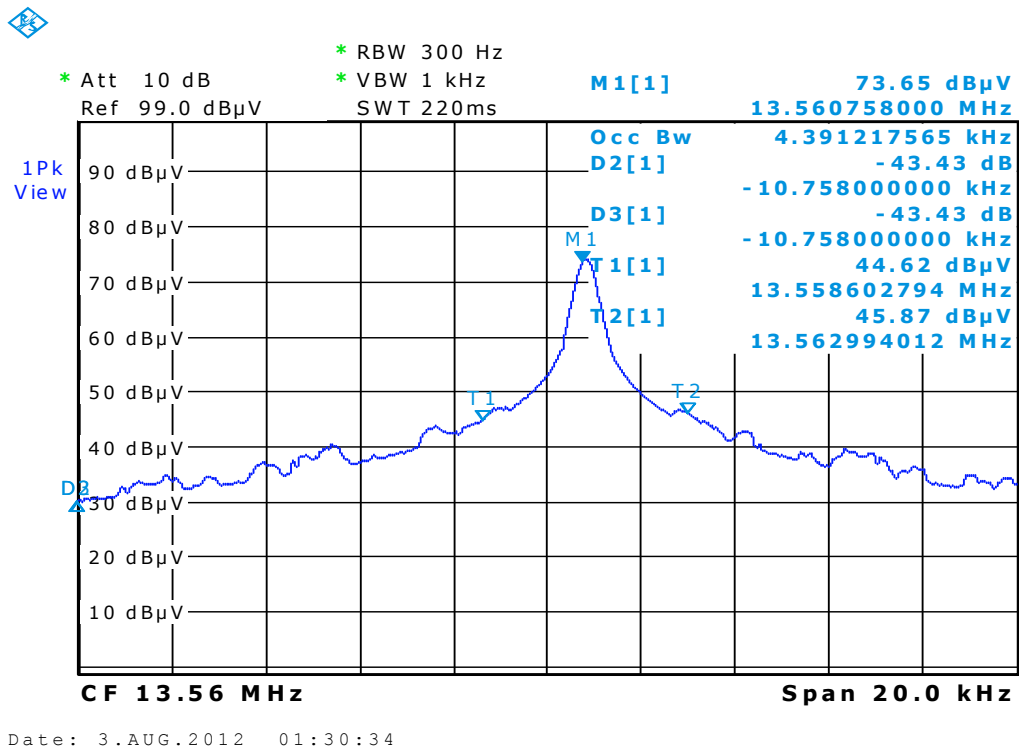
Plots: 13.56 MHz
