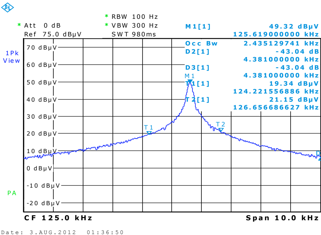
Plots: 125KHz
