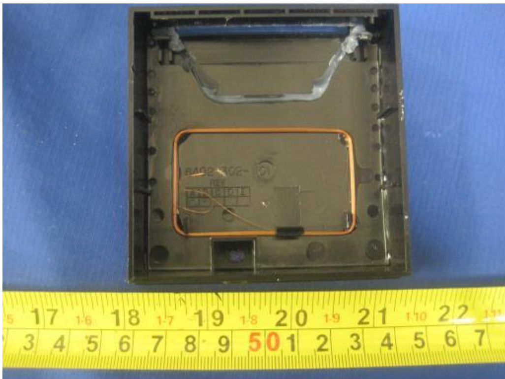
Loop Antenna (Terminal Connector)
