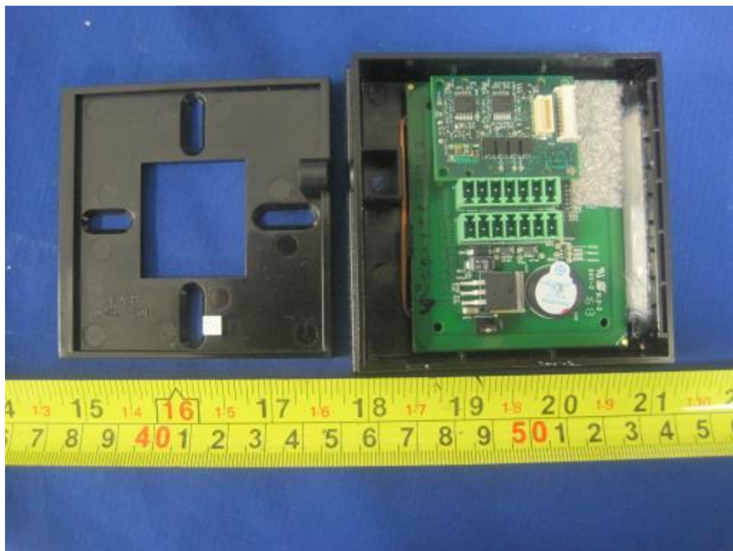
Cover off View (Terminal Connector)
