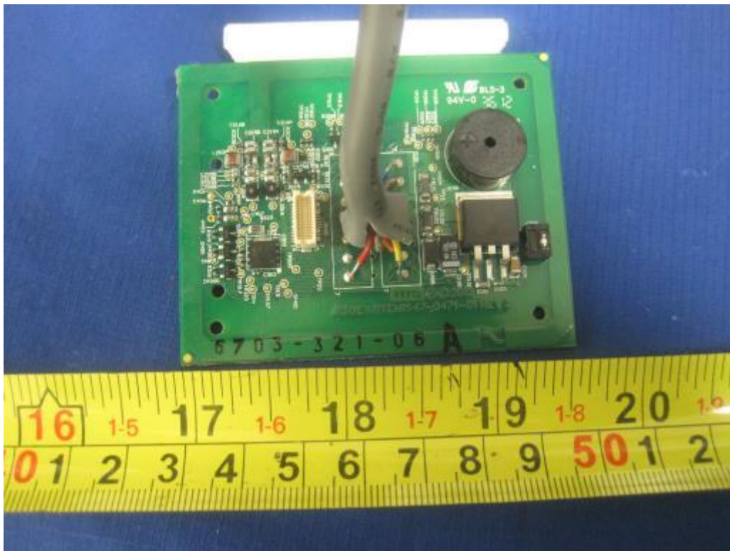
Main PCBA Bottom View (Pigtail Connector)
