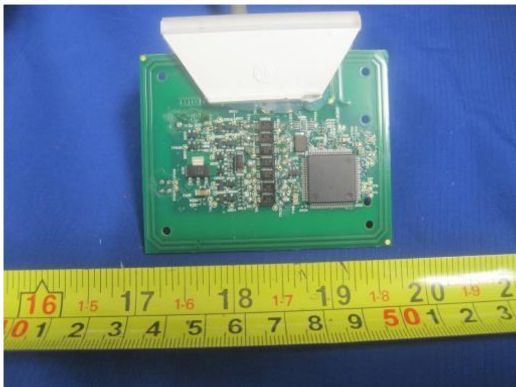
Main PCB Top View (Pigtail Connector)
