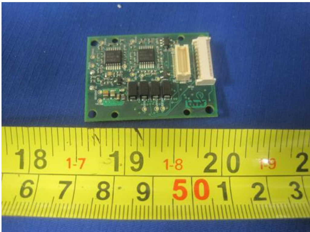
Sub PCBA Top View (Terminal Connector)
