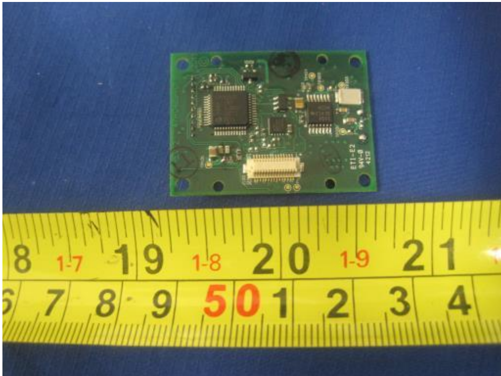
Sub PCBA Bottom View (Terminal Connector)
