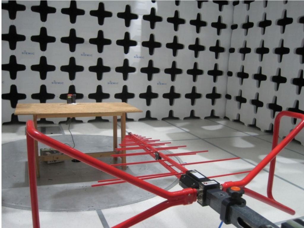
Terminal cable Radiated Emission>30MHz Test Setup – Front View
