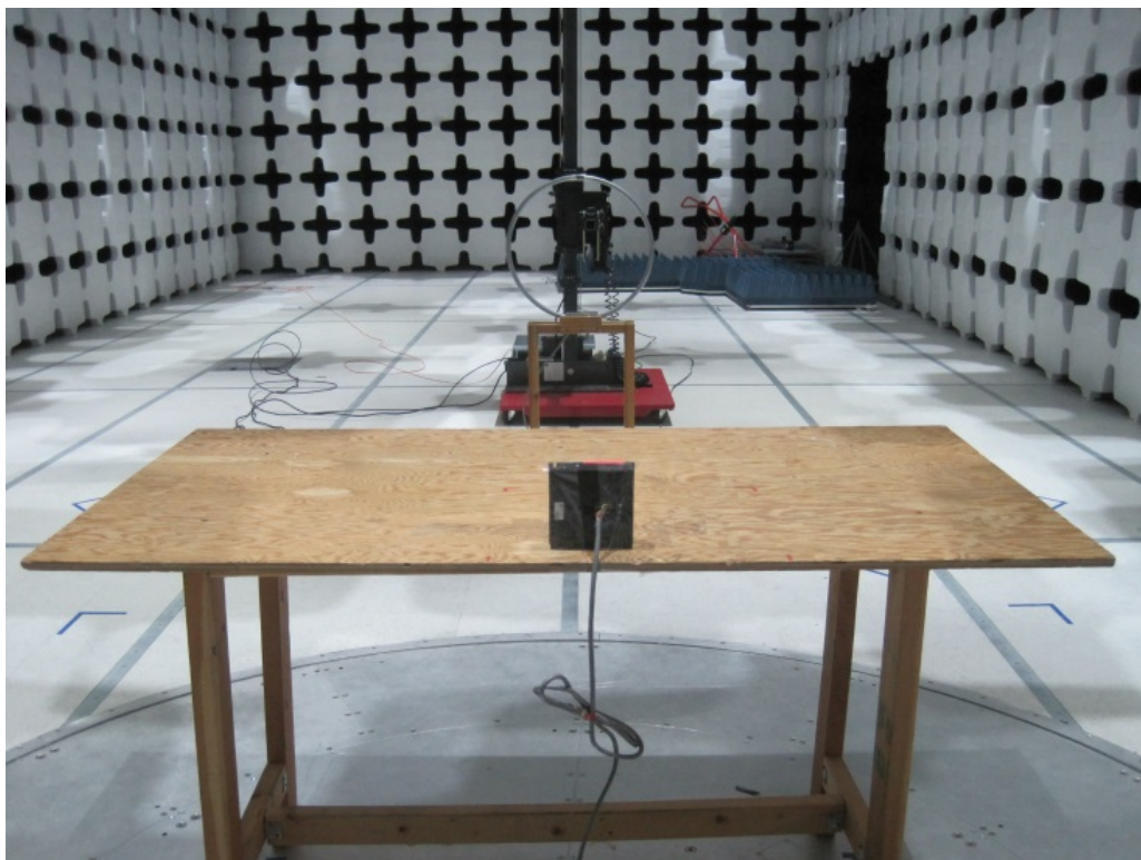
Terminal Radiated Emission<30MHz Test Setup – Rear View
