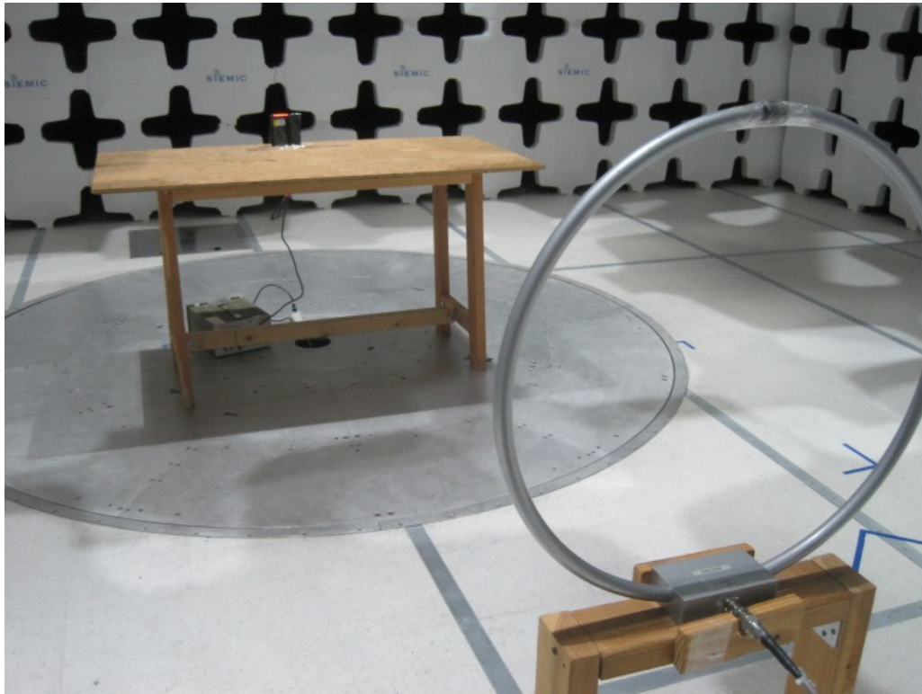
Terminal Radiated Emission<30MHz Test Setup – Front View
