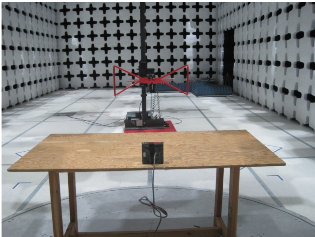
Terminal cable Radiated Emission>30MHz Test Setup – Rear View
