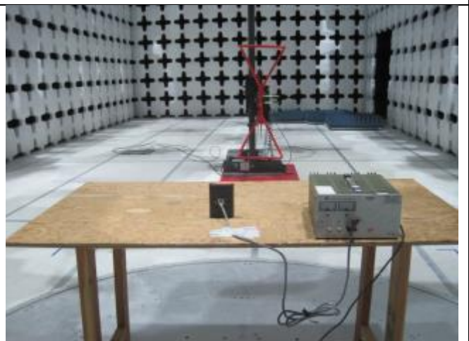
Radiated Emissions (<1GHz) – Rear View (Terminal Connector)
