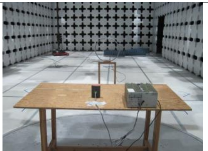
Radiated Emissions (<30MHz) – Rear View (Terminal Connector)
