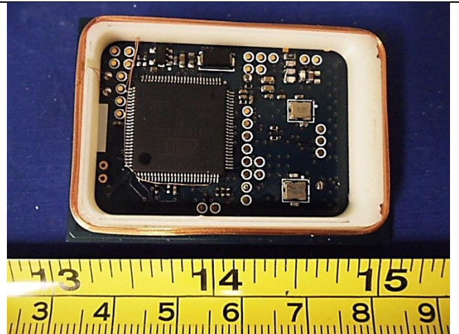
PCBA View 2
