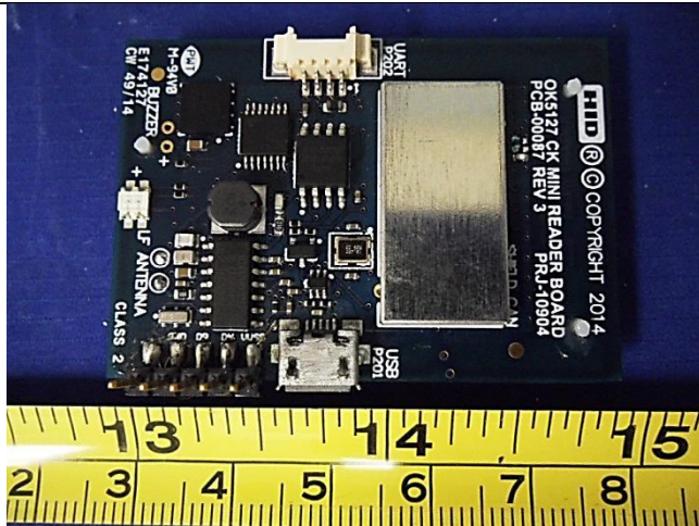
PCBA View 1
