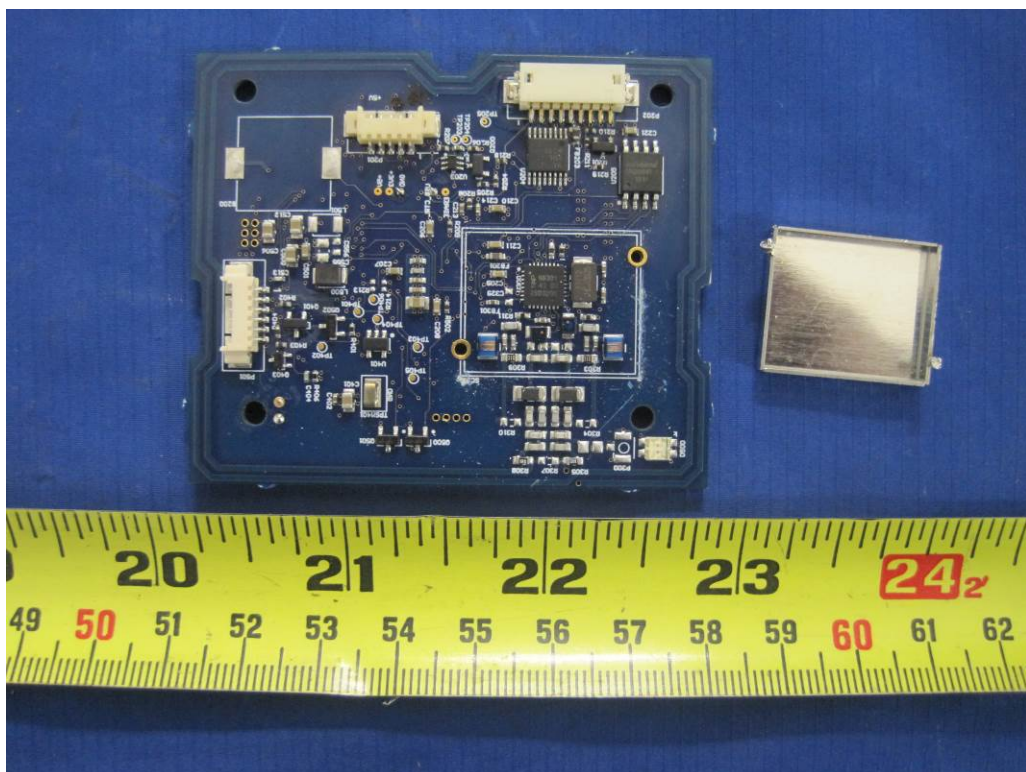
EUT Top View with Shield Removed
