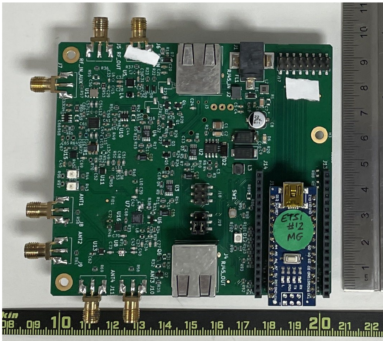
Top view, RF booster
