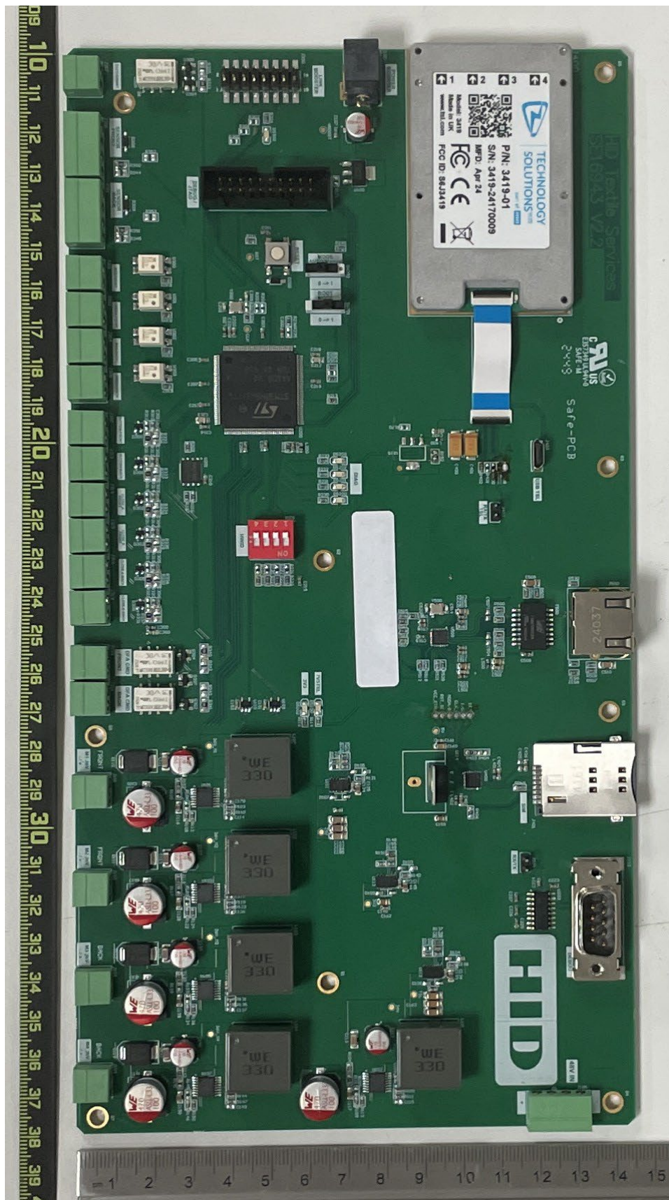
Top view with RF module, controller
