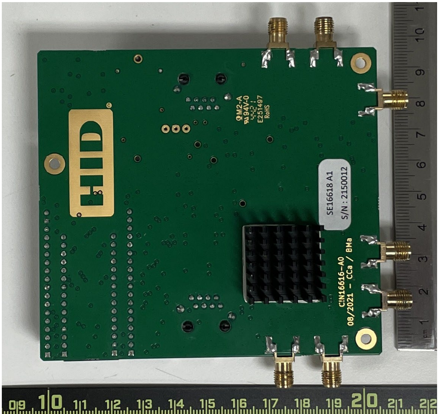
Bottom view, RF booster
