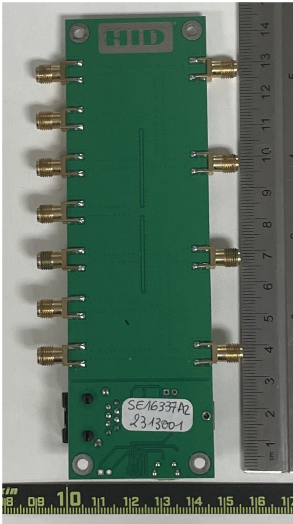
Bottom view, RF extractor
