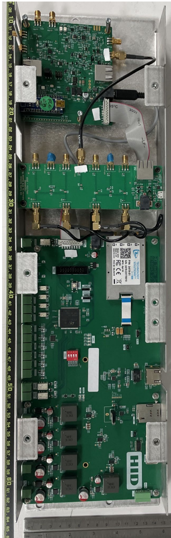
RF assembly with controller, RF module, RF extractor and RF booster
