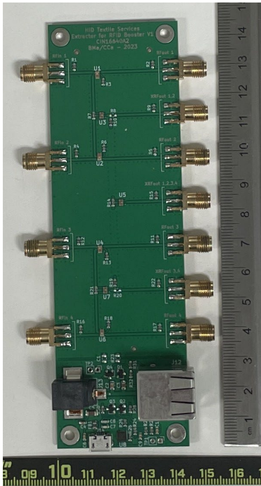
Top view, RF extractor
