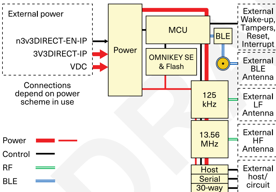
OMNIKEY SE Reader Core block diagram
