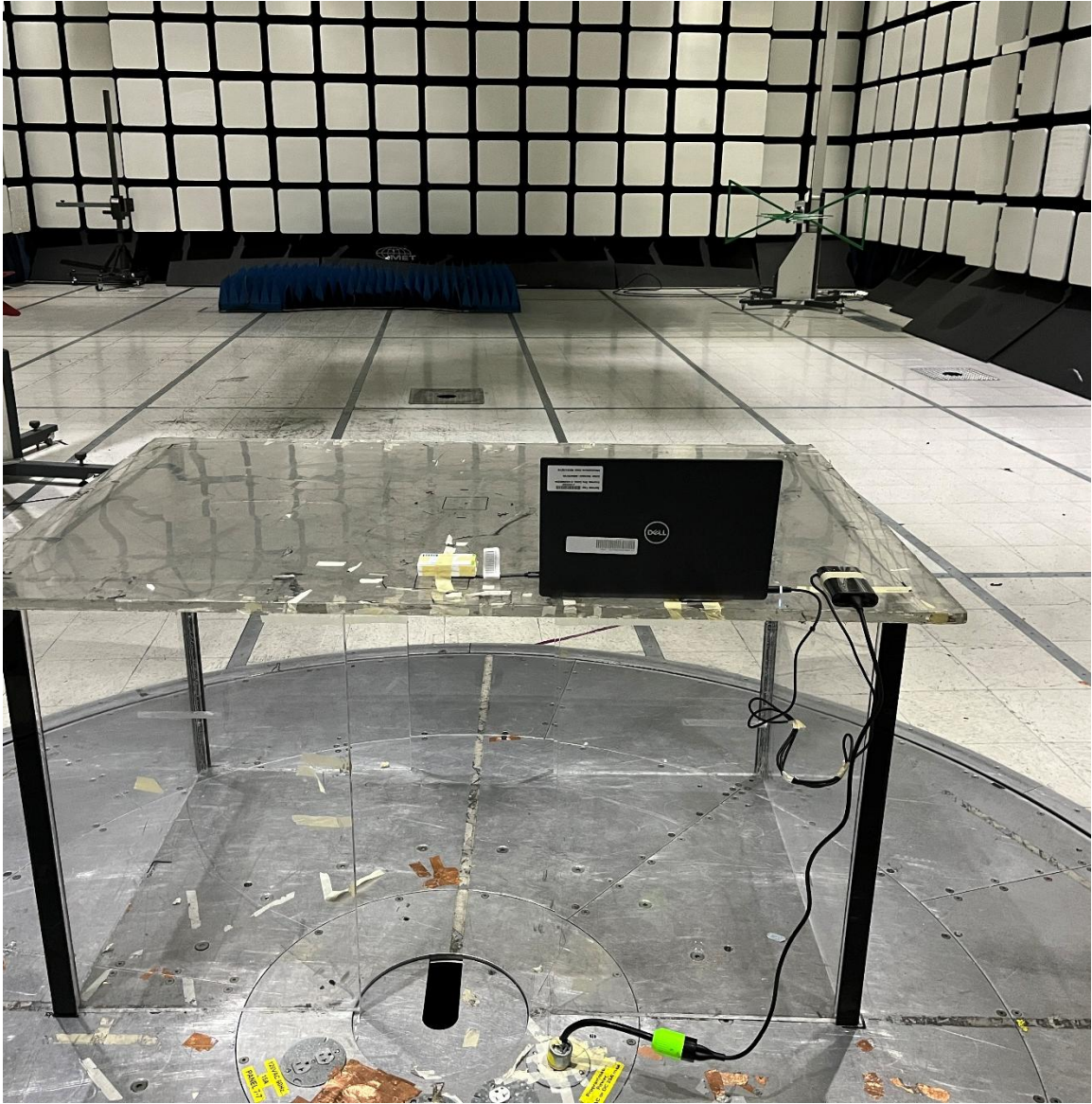
Radiated Emissions (30MHz – 1GHz)
