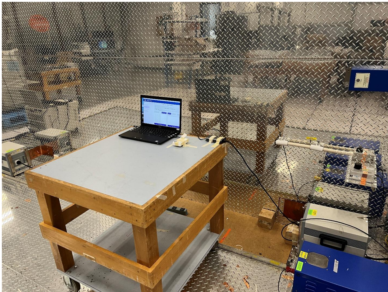
Conducted Emissions at AC Mains of the PC
