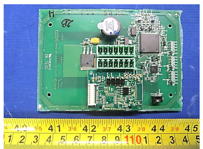
PCBA 1 Top View 2 with PCBA2
