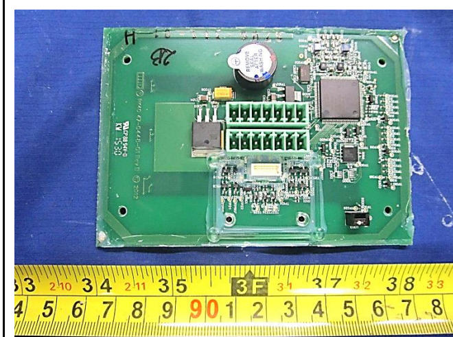
PCBA 1 Top View 1 without PCBA2
