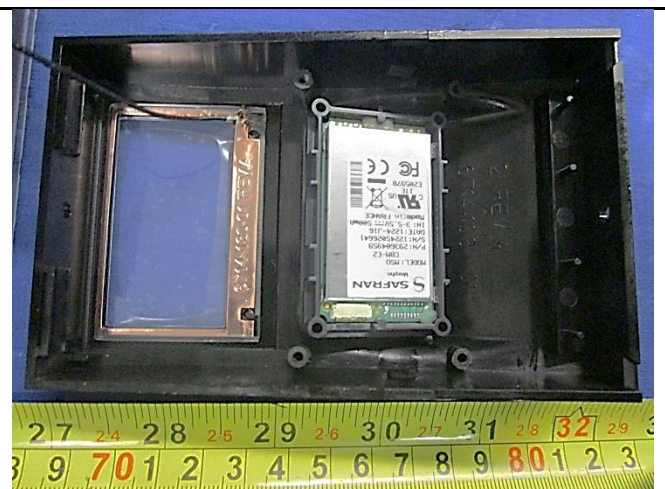
Cover off View 4
