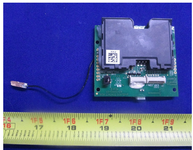
PCBA3 Bottom View
