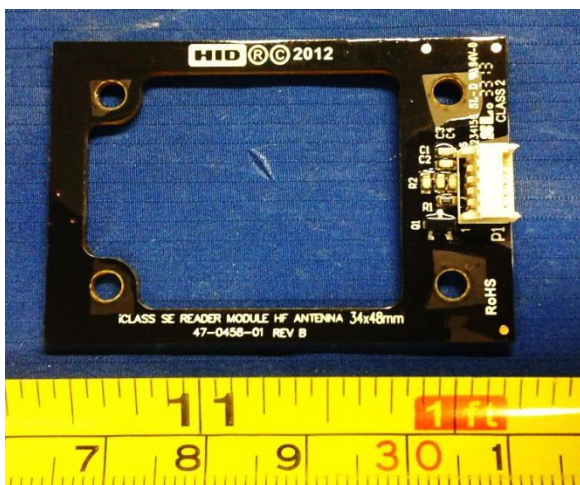
High Frequency Short Antenna Top View
