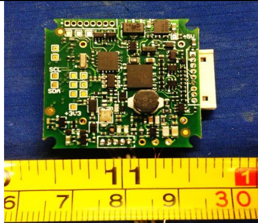
SE3200 Bottom View
