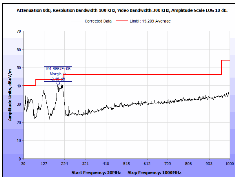
Figure 109: Radiated Spurious Emissions, Terminal, 2480 MHz, 30 MHz – 1000 MHz, Vertical
