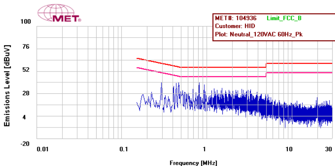
Figure 13: Conducted Emissions Limits, Pigtail, Neutral Line, Prescan
