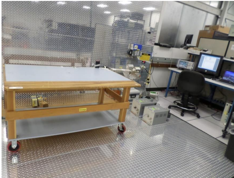
Figure 3: Conducted Emissions Limits, Pigtail, Test Setup, Front View
