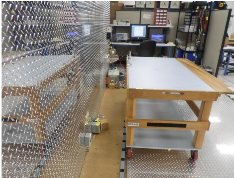
Figure 4: Conducted Emissions Limits, Pigtail, Test Setup, Back View
