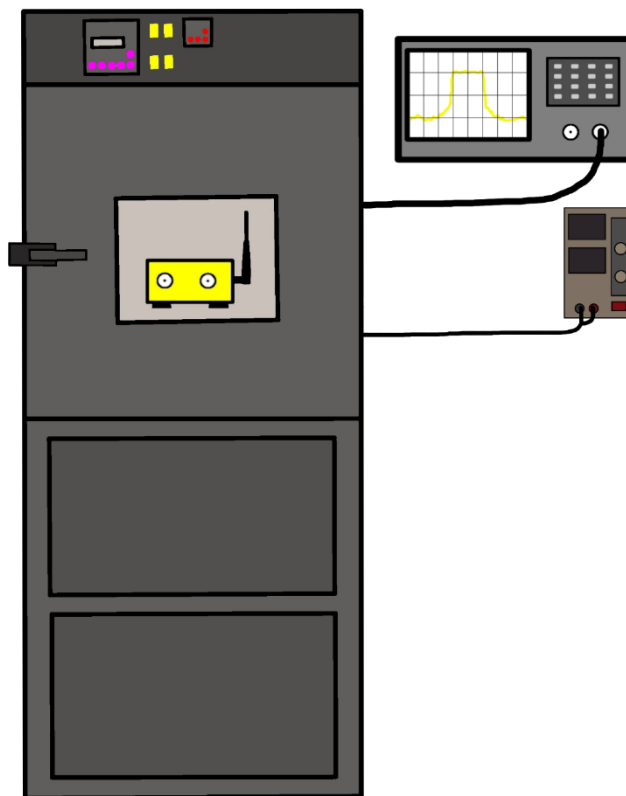
Figure 7. Temperature Stability Test Setup
