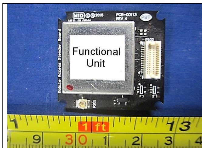
Module View 1
