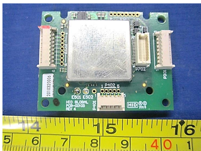
SE3210 Host View 1
