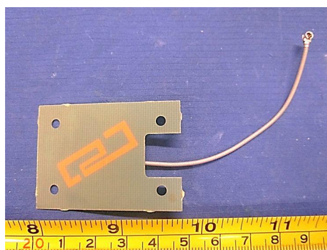
Antenna View 2
