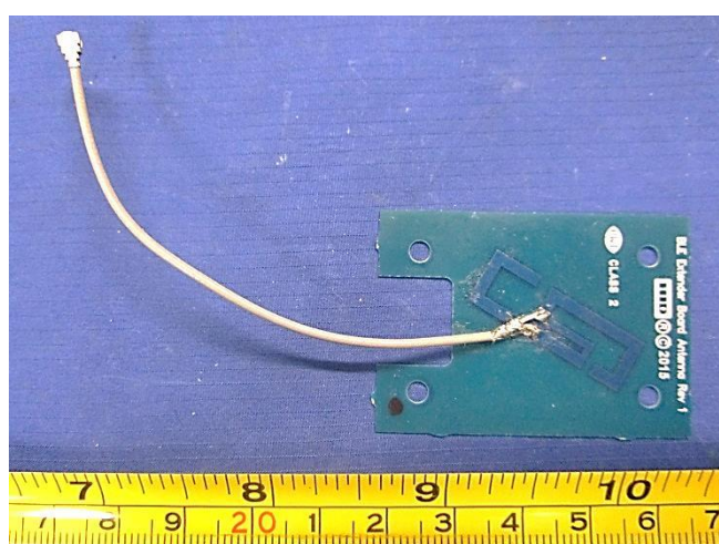
Antenna View 1
