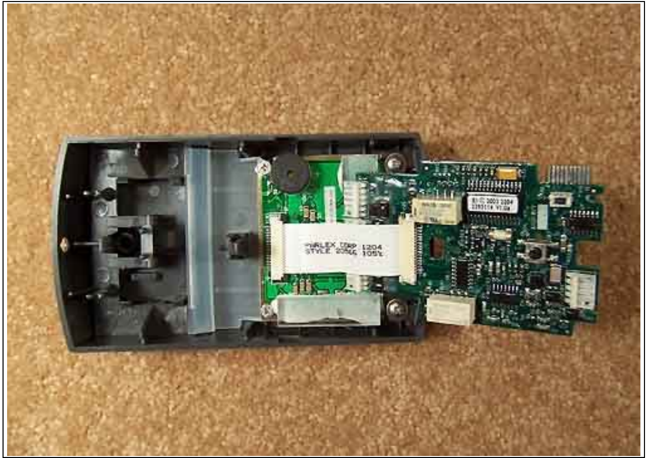
Internal PCB Connection - Remote Antenna
