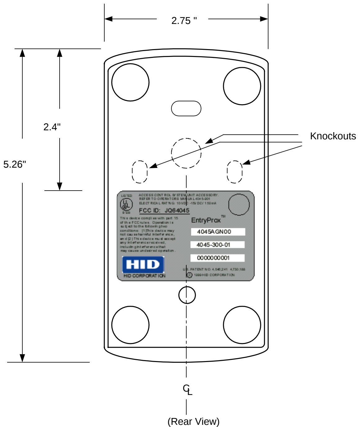
FCC Label Location for HID Corp Model 4045A EntryProx
