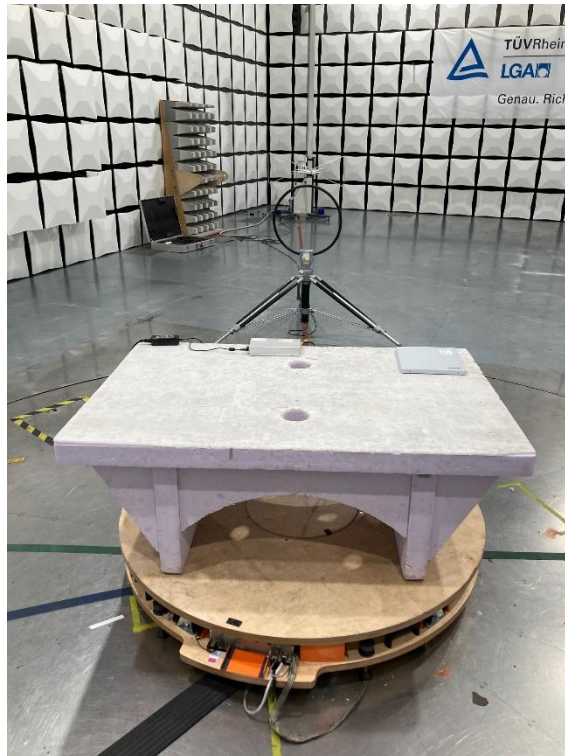
Test Setup: Radiated Measurements (9 kHz - 30 MHz)
