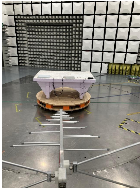
Test Setup: Radiated Measurements (30 MHz - 1 GHz)
