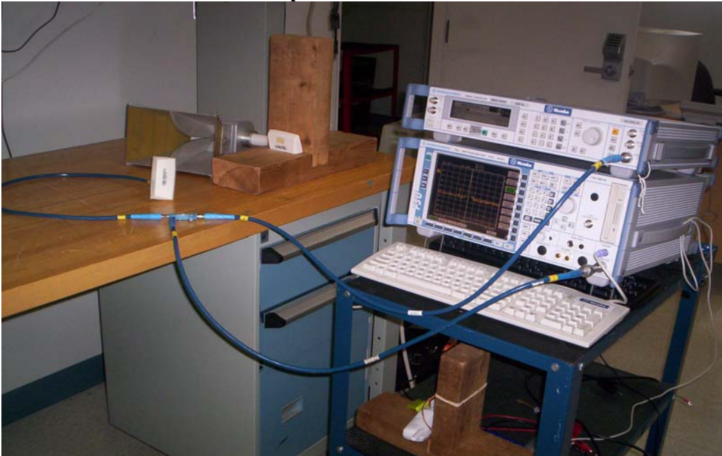
Conducted Measurement Setup:
