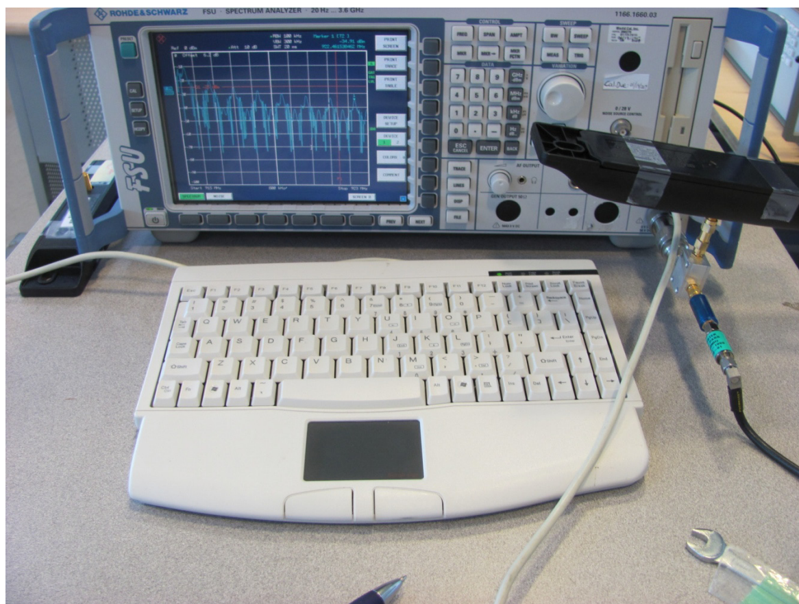
Illustration 3: Antenna conducted emission setup
