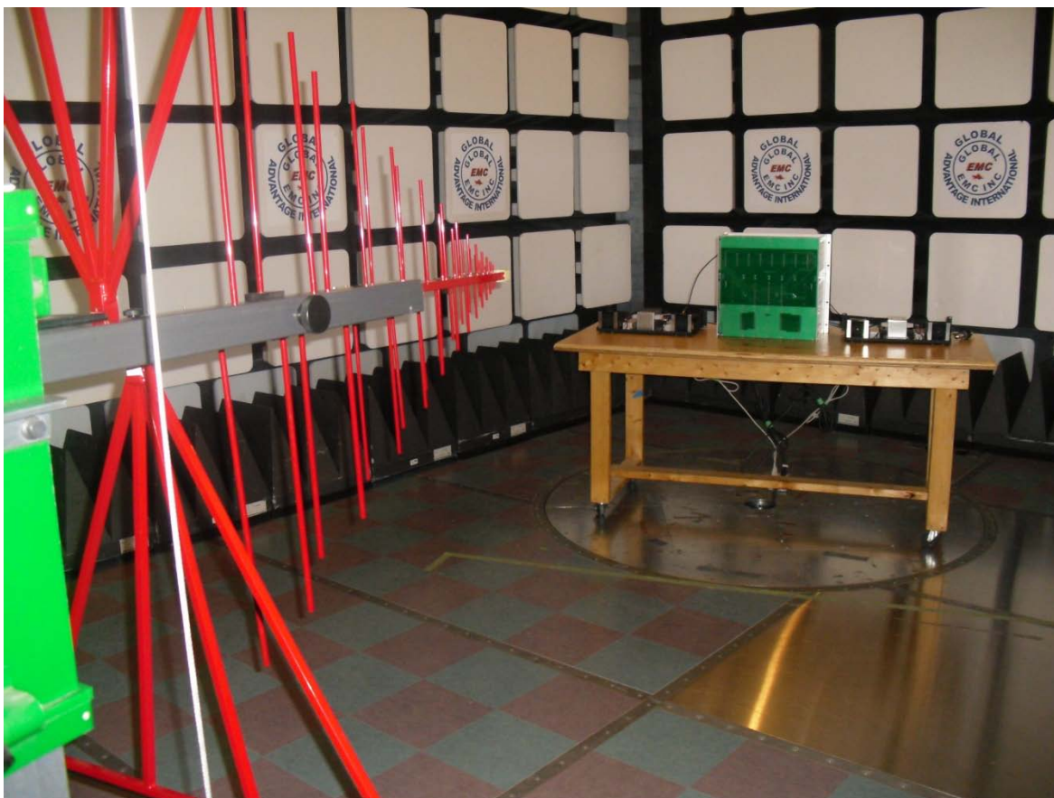
Illustration 1: 802295A-A Radiated emission setup – photo 1 Note: 4 instances of 802295A-A were present in setup
