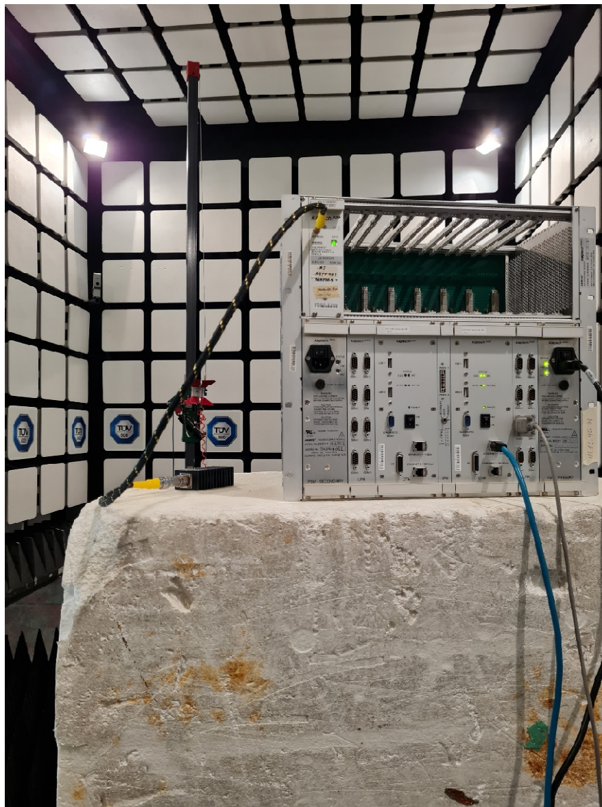
Figure 1 – Radiated Emissions Setup – Photo 1
