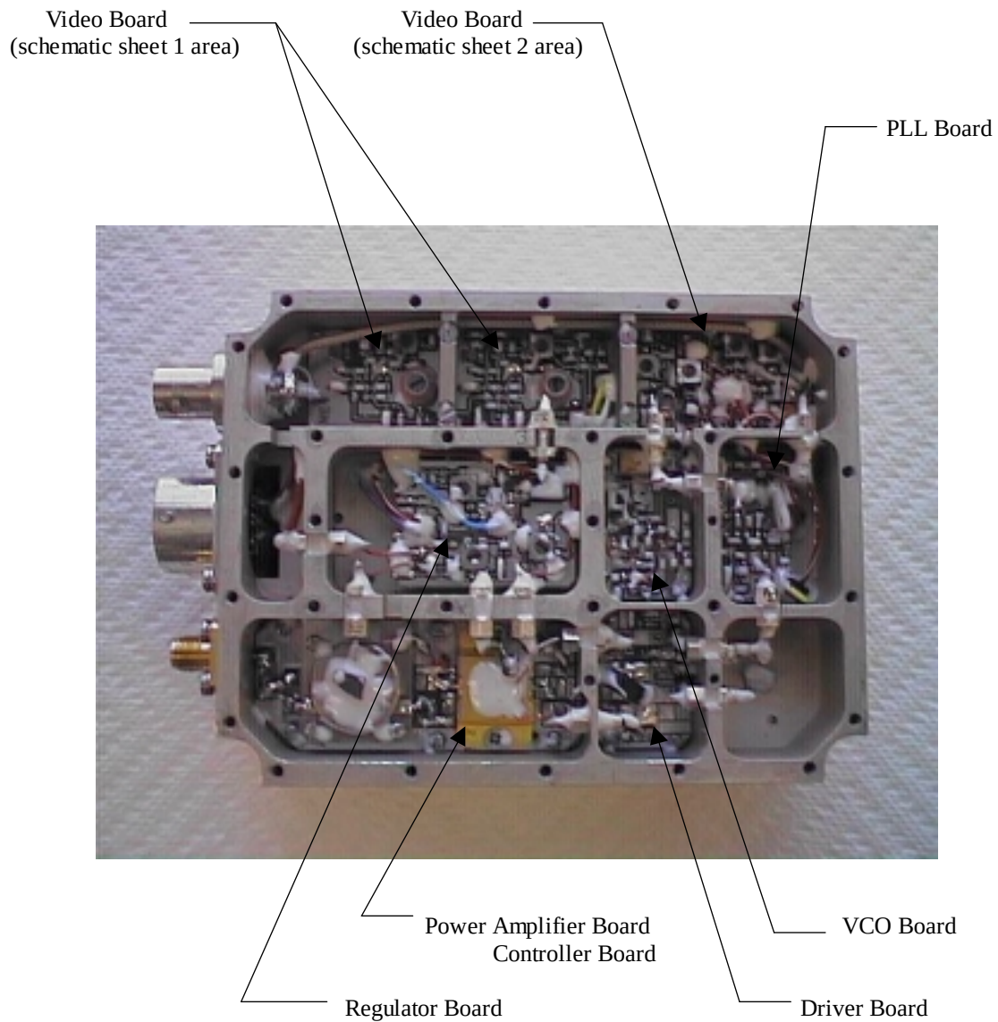
TRANSMITTER BOTTOM VIEW
