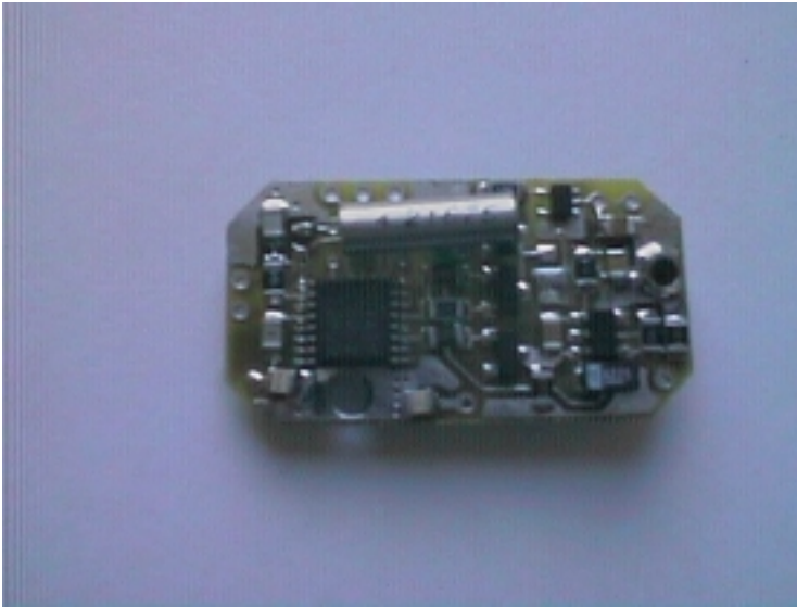
PLL BOARD- TOP VIEW
