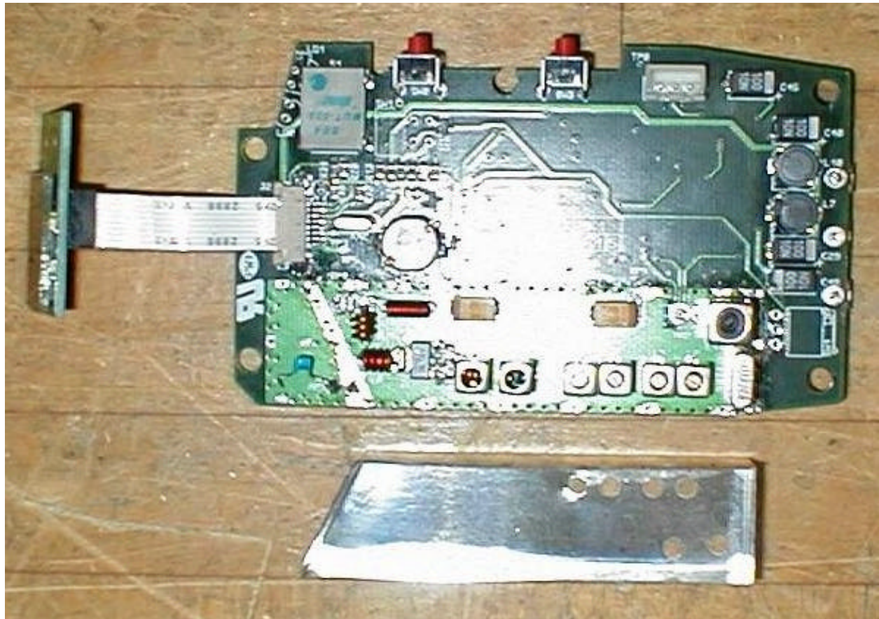
PCB Bottom, Shield Removed View
