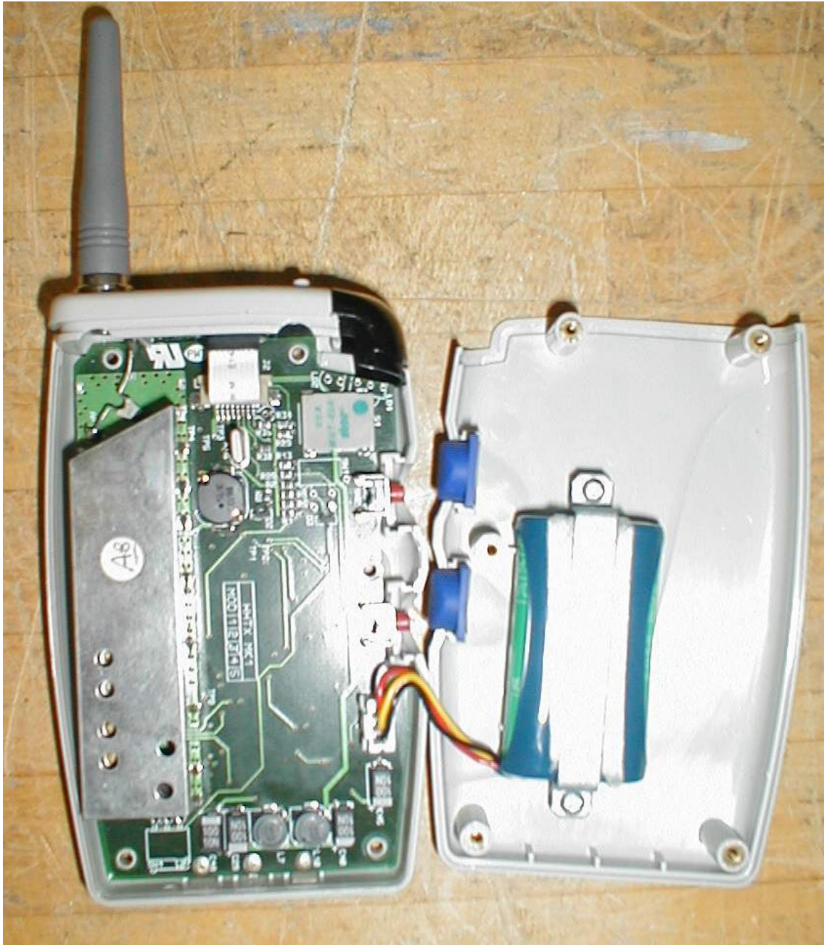
EUT, Cover Removed
