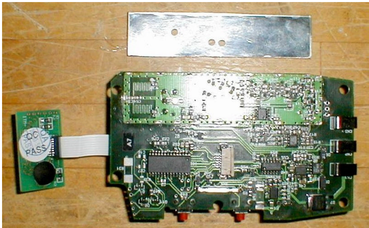
PCB Bottom, Shield Removed View
