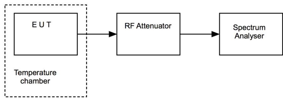
Figure v Test Setup
