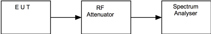
Figure viii Test Setup
