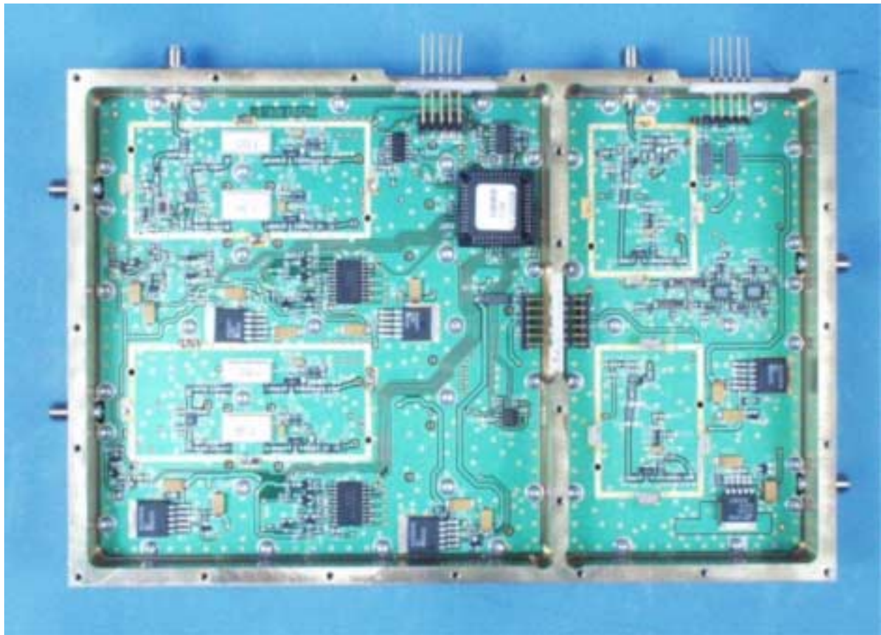
Module B, Top w/o shields
