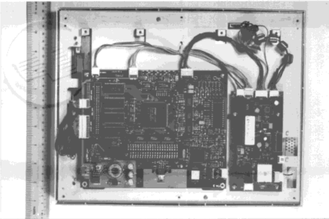
EUT Internal View - Inner Metal Casing Removed
