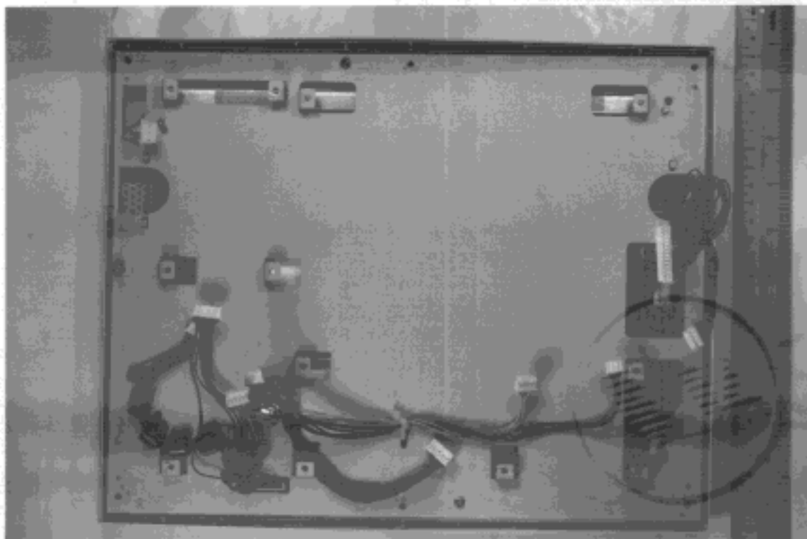
EUT Internal View - EUT PCBs Removed
