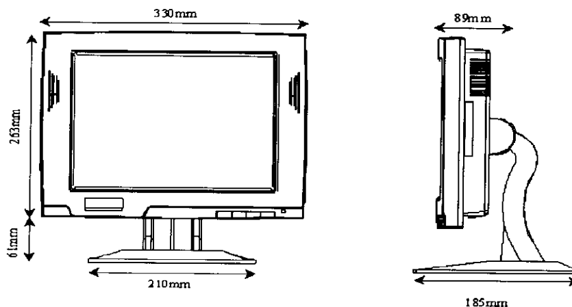
Figure 4 Dimensions of the LCD monitor
