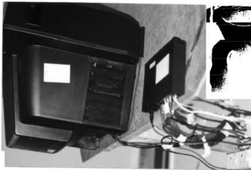
Figure 6. Conducted emissions test setup (back view)
