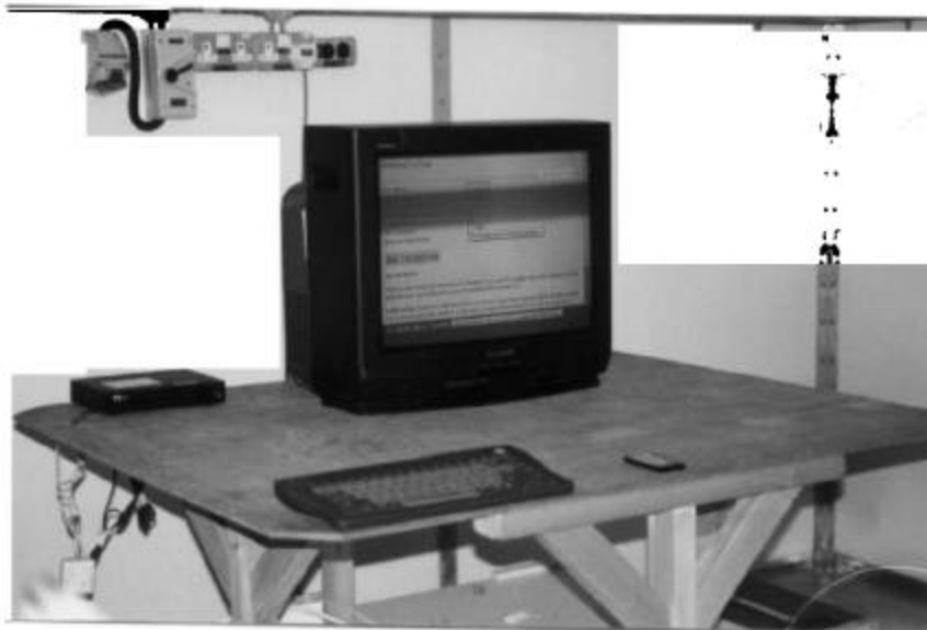
Conducted emissions test setup (front view)
