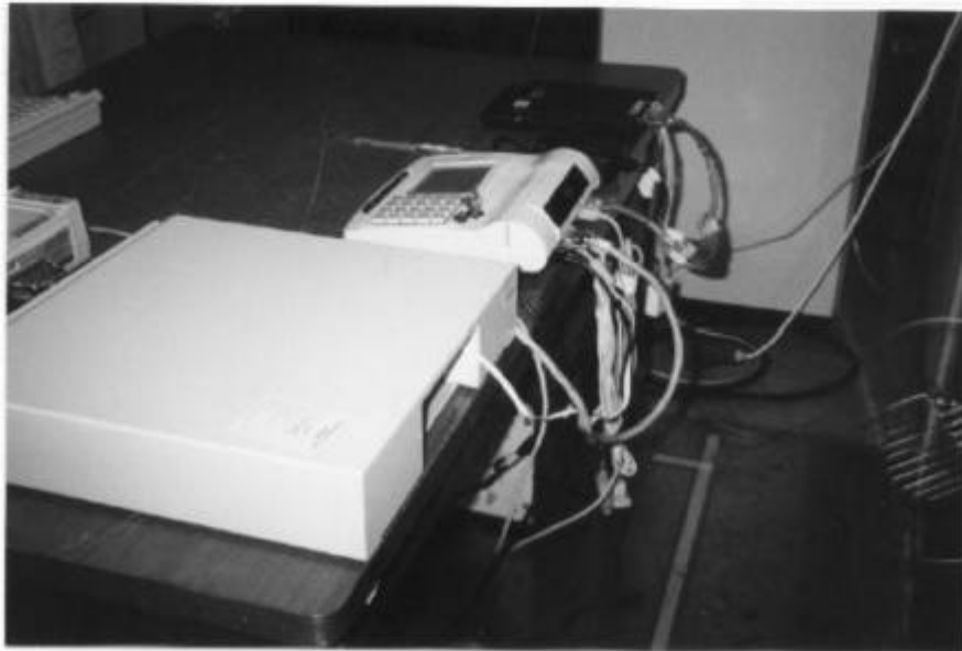
Conducted Emissions Test Setup – Rear View
