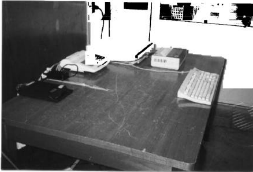
Conducted Emissions Test Setup – Front View
