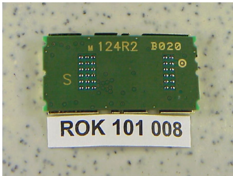
Picture 3 : Bottom side of module (with case)
