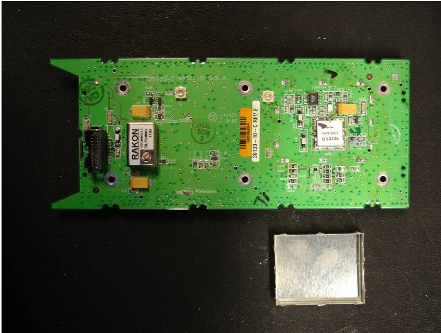
EUT – Internal PCBA View 3
