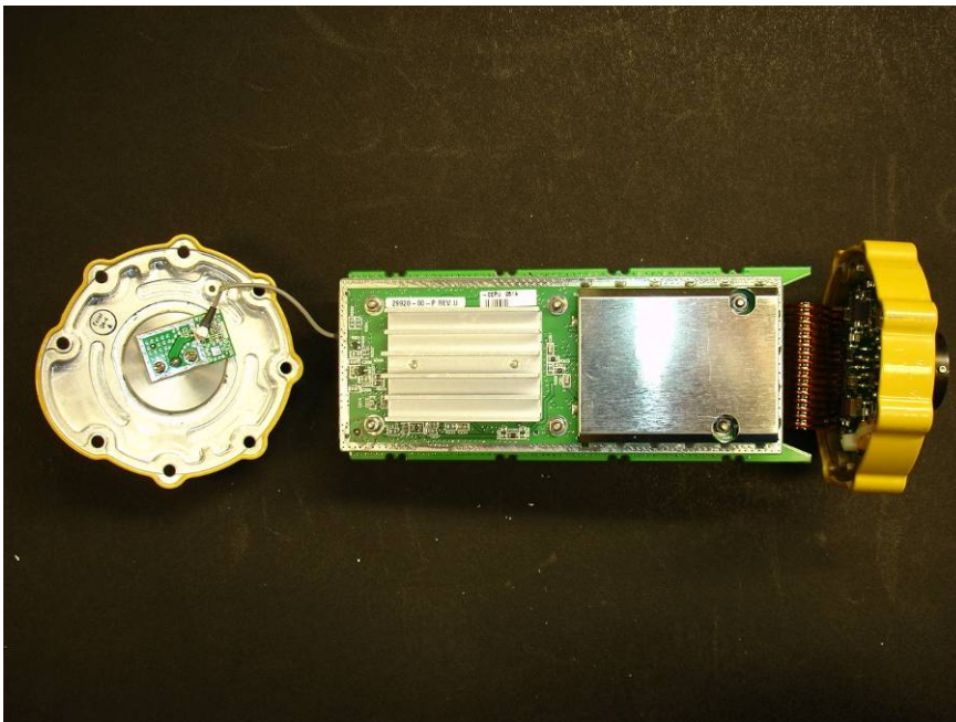
EUT – Internal PCBA View 2
