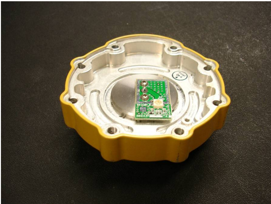
EUT – Antenna PCBA and Cap
