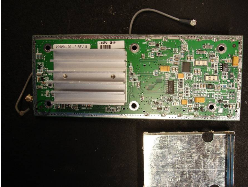
EUT – Internal PCBA View 5
