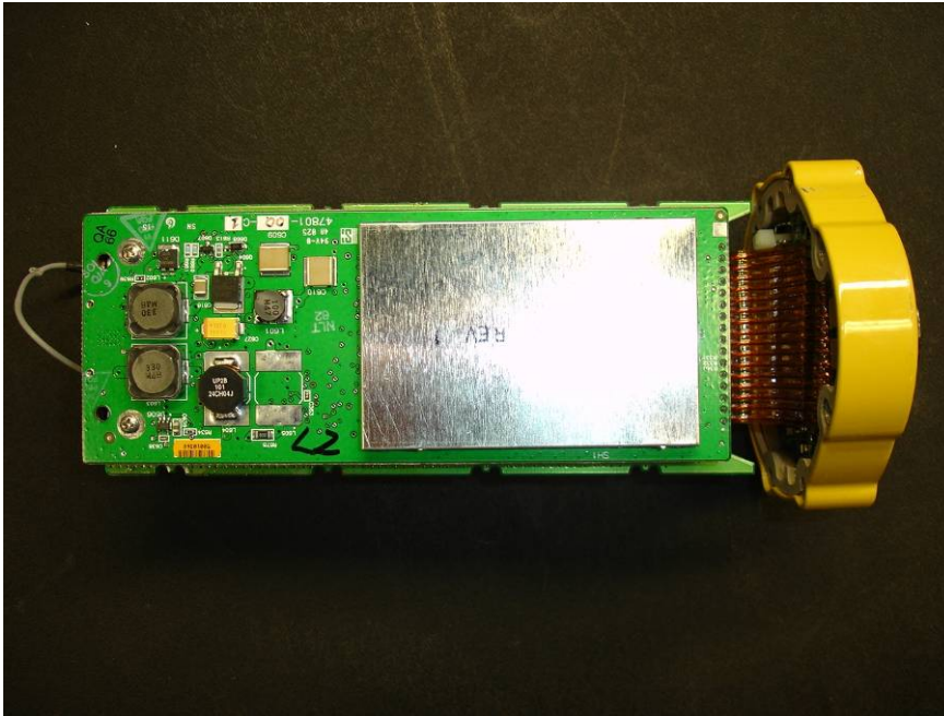
EUT – Internal PCBA View 1
