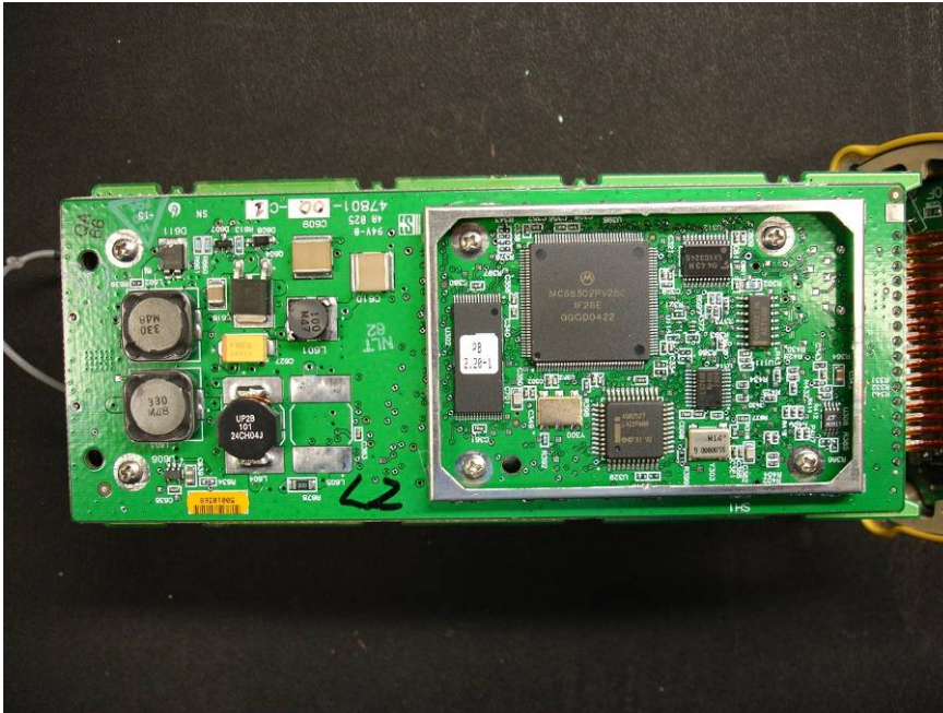
EUT – Internal PCBA View 7
