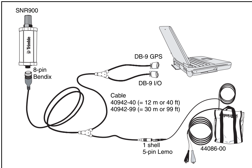
Figure 4.10 Machine service cable (PN 40942-xx)
