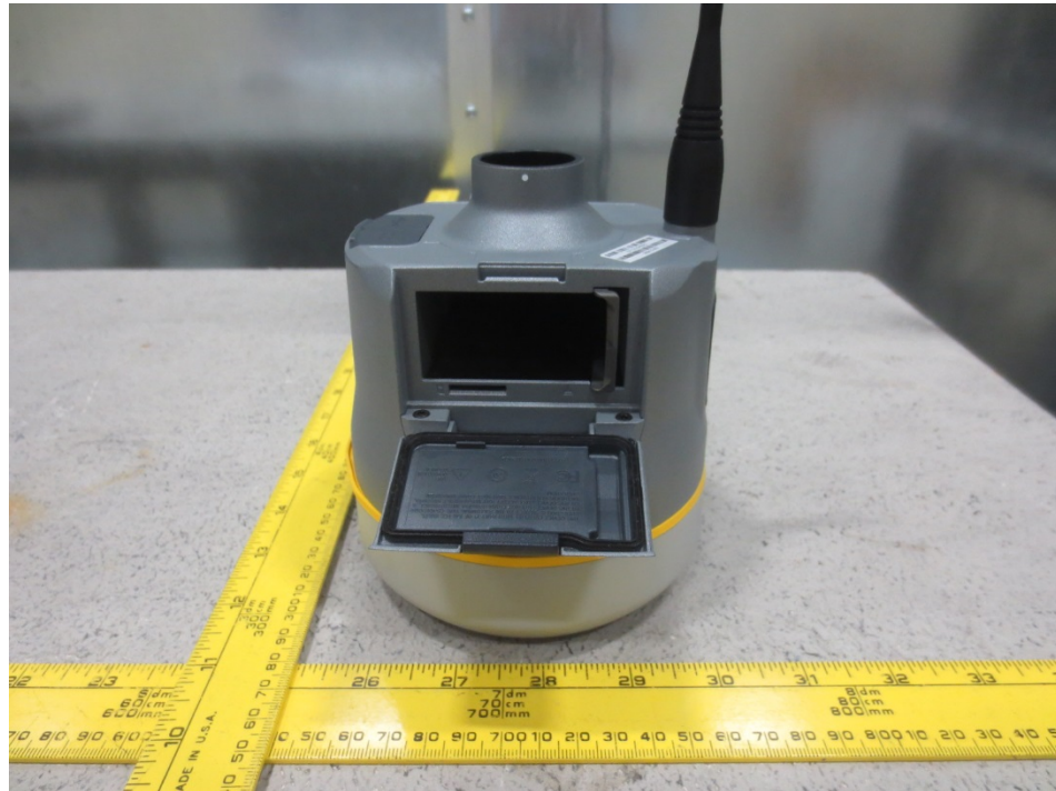
Host Device - Open Cover View-2
