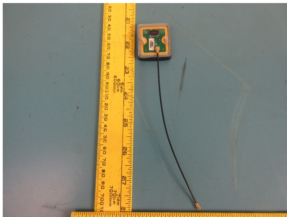
WiFi/BT Patch antenna from Host R10-2 View
