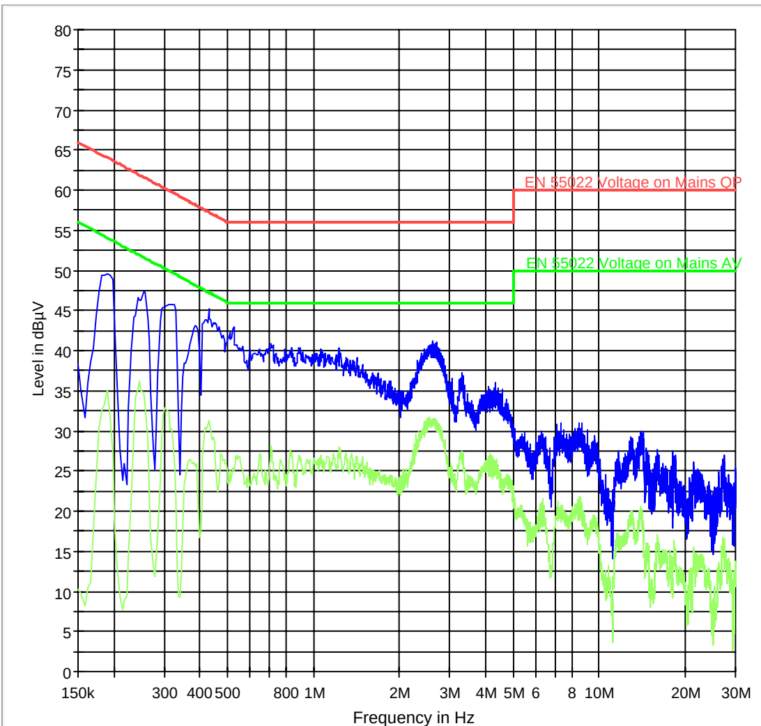
CISPR 22 Mains Conducted
