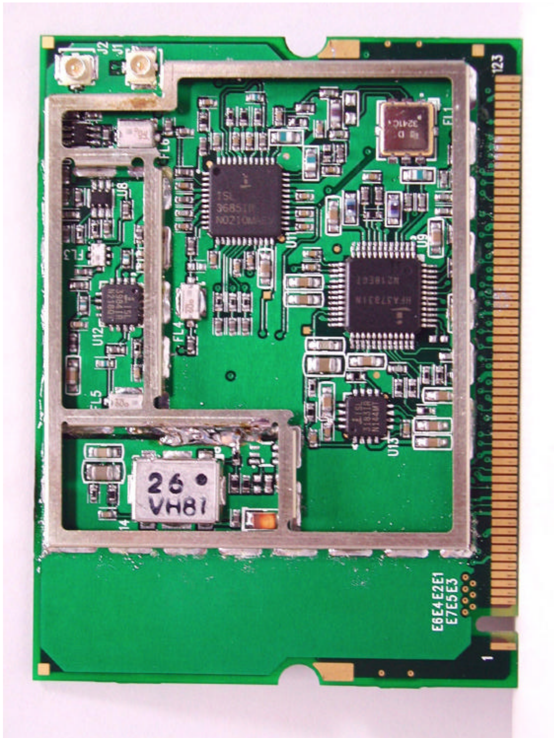
FCC ID: JVPAWL200 RF module of the PWBA
