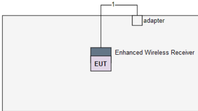
Test Setup Diagram (Charging Mode)
