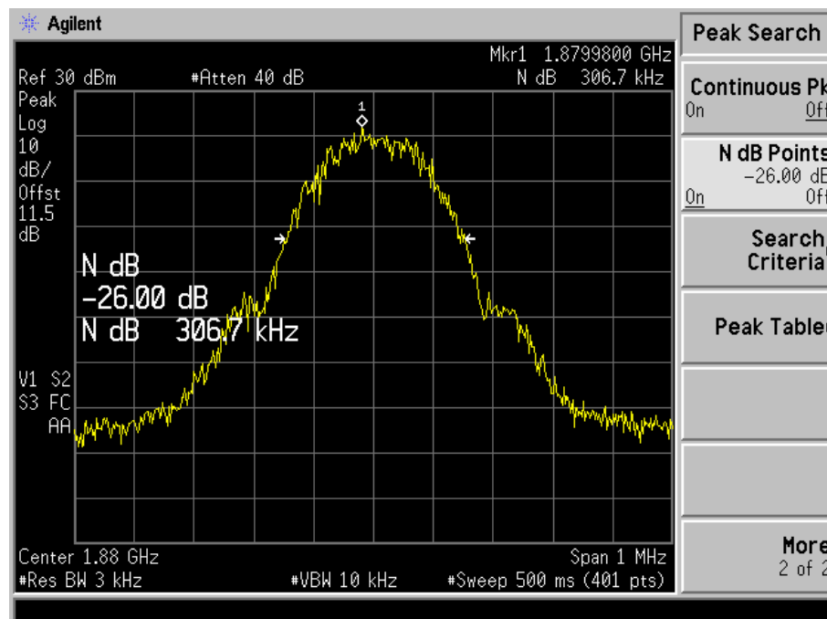
Packet Switched (GPRS Mode CH661)
