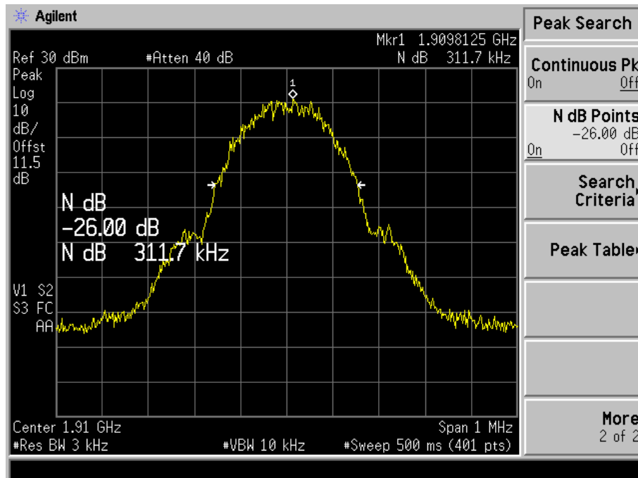
Packet Switched (GPRS Mode CH810)
