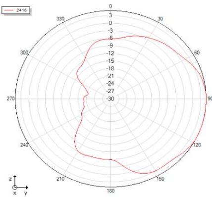
Phi=90 freq=2416MHz
