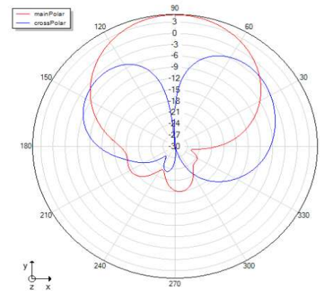
Theta=90 freq=2434MHz
