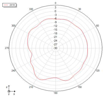
Phi=0 freq=2416MHz
