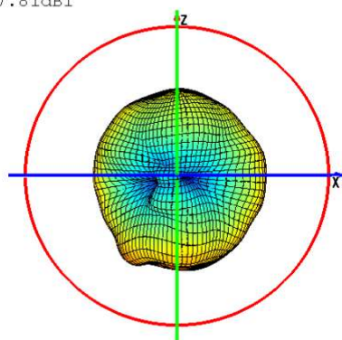
Phi=0 freq=2454MHz
