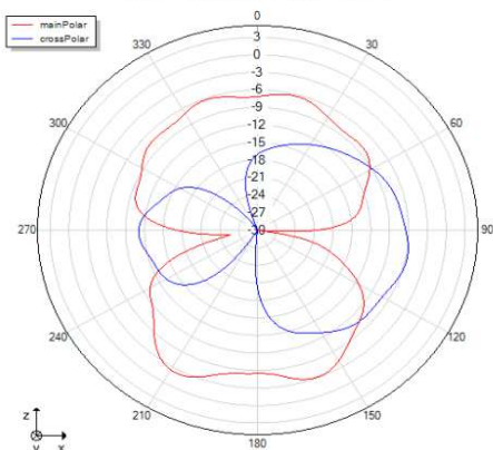
Phi=0 freq=2402MHz
