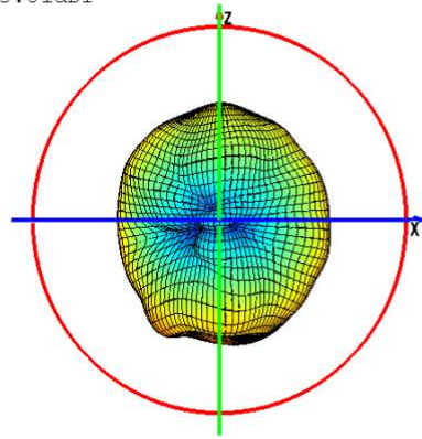
Phi=0 freq=2440MHz
