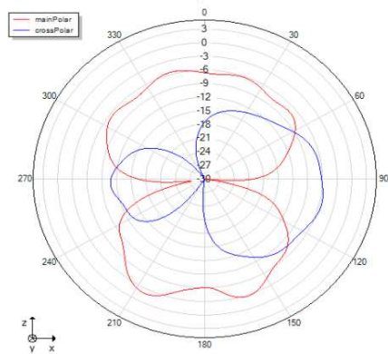
Phi=0 freq=2416MHz
