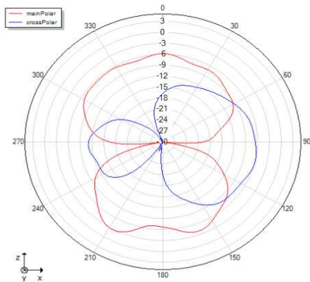
Phi=0 freq=2434MHz
