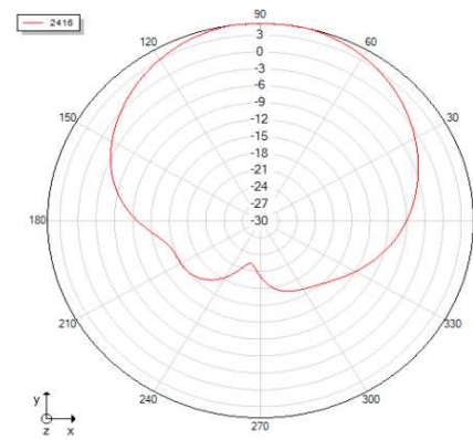
Theta=90 freq=2416MHz
