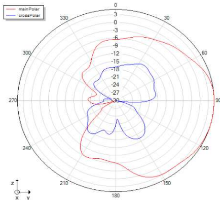
Phi=90 freq=2422MHz
