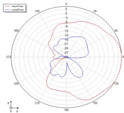
Phi=90 freq=2416MHz
