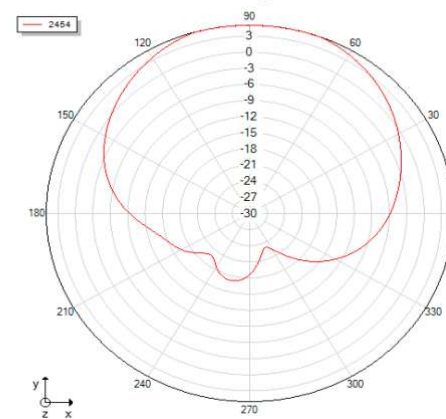
Theta=90 freq=2454MHz
