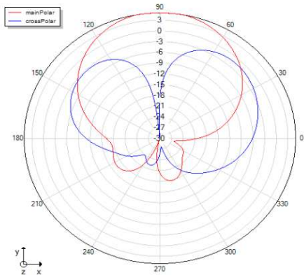
Theta=90 freq=2422MHz
