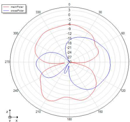
Phi=0 freq=2454MHz
