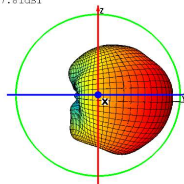
Theta=90 freq=2454MHz
