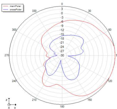
Phi=90 freq=2454MHz
