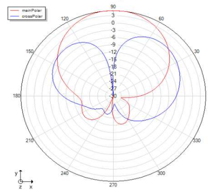
Theta=90 freq=2416MHz
