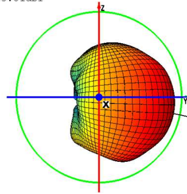
Theta=90 freq=2440MHz
