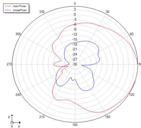
Phi=90 freq=2434MHz
