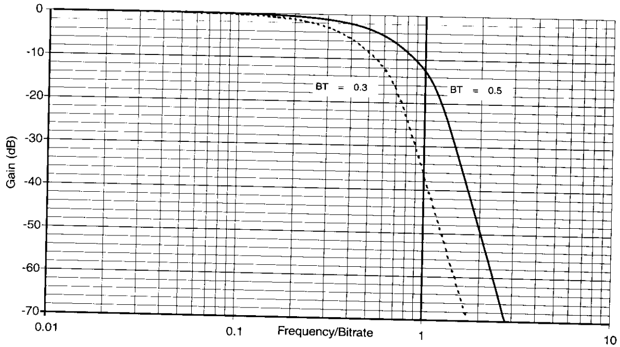
Figure 9: Tx Filter Response
