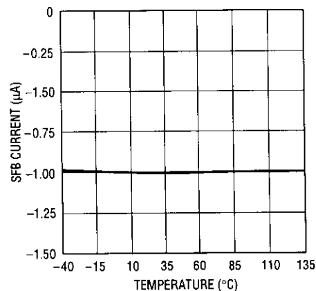
SFB1 Pin Current vs Temperature
