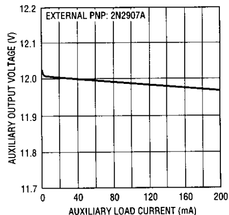
Auxiliary Regulator Load Regulation
