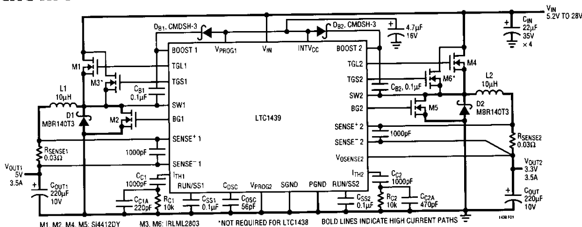
Figure 1. High Efficiency Dual 5V/3V Step-Down Converter
