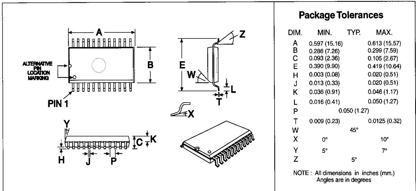
Figure 30: 24-pin SOIC Mechanical Outline: Order as part no. MX919BDW
