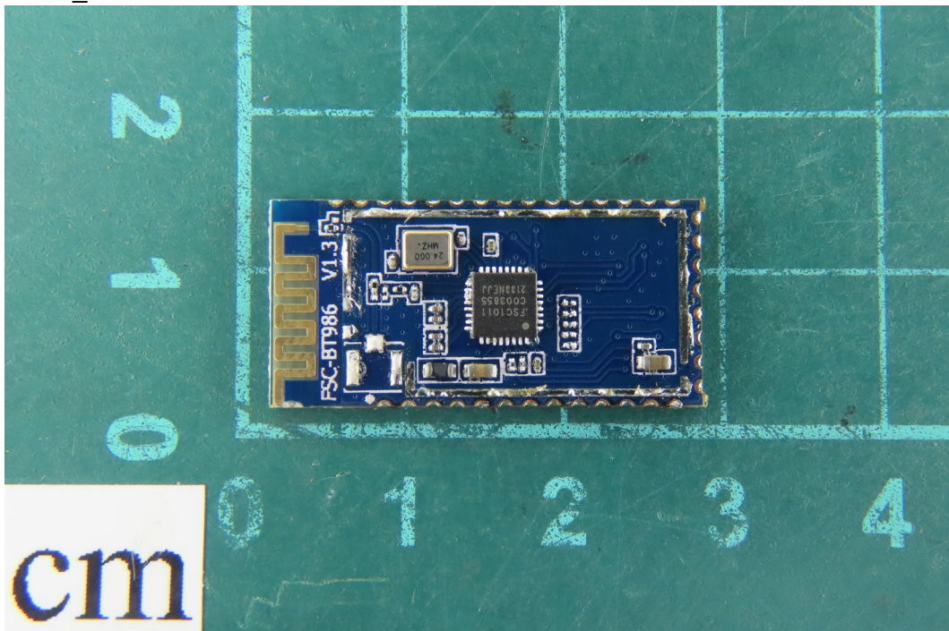
(28) EUT Photo_Bluetooth Module + Ant
