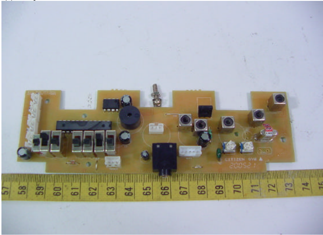
(6) Component View of PCB
