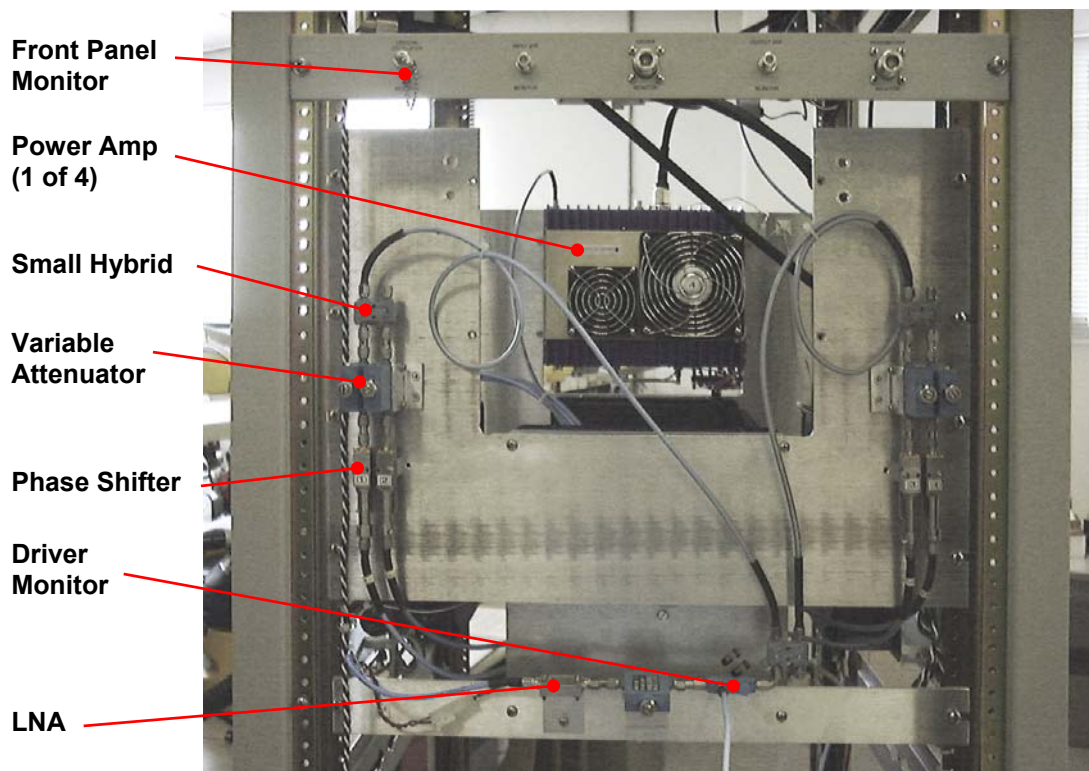
Figure 10. Front Internal View.
