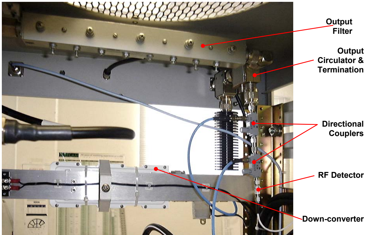
Figure 9. ITX02-2000 Internal View (looking rear, upper right).
