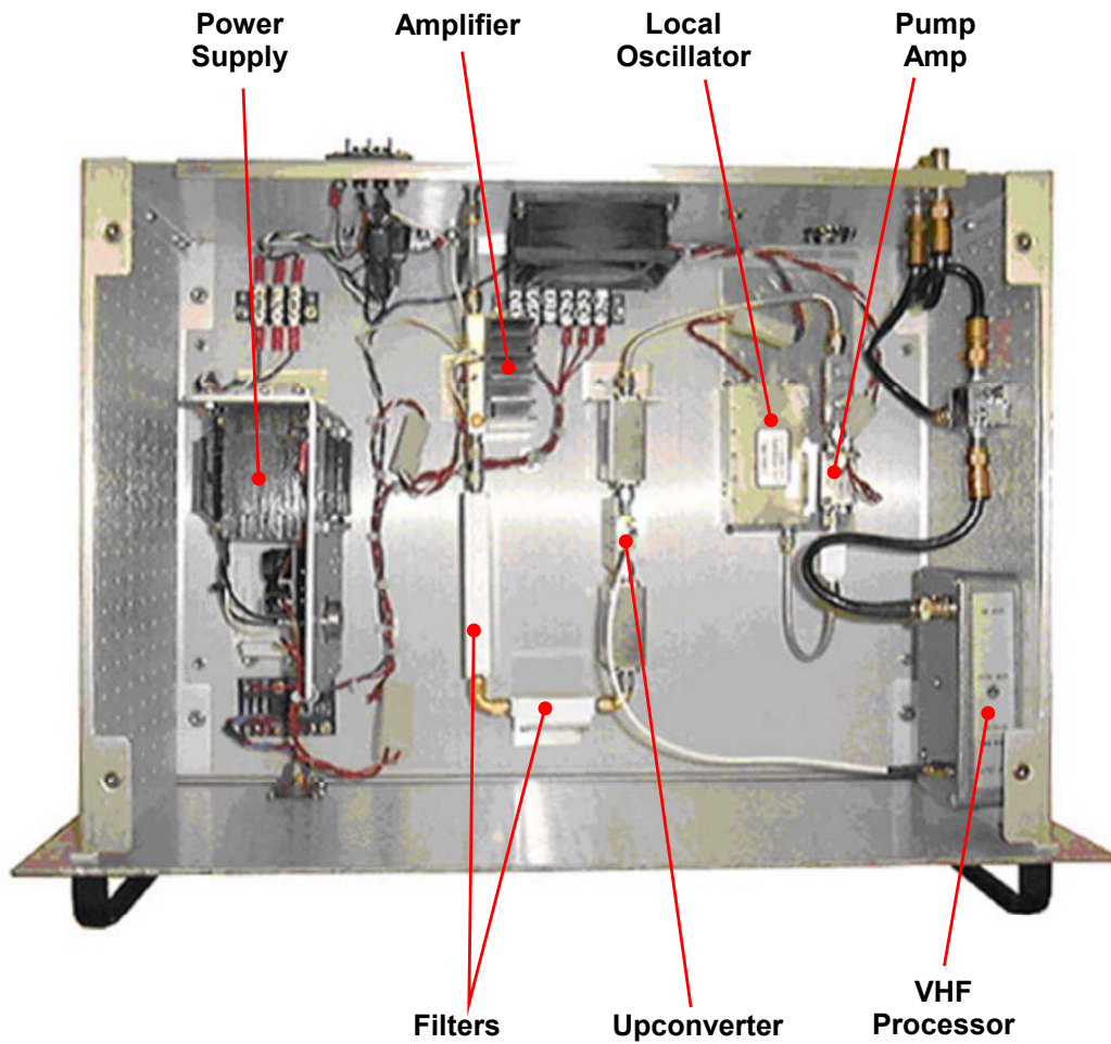
Figure 15. Driver Chassis Component Layout.
