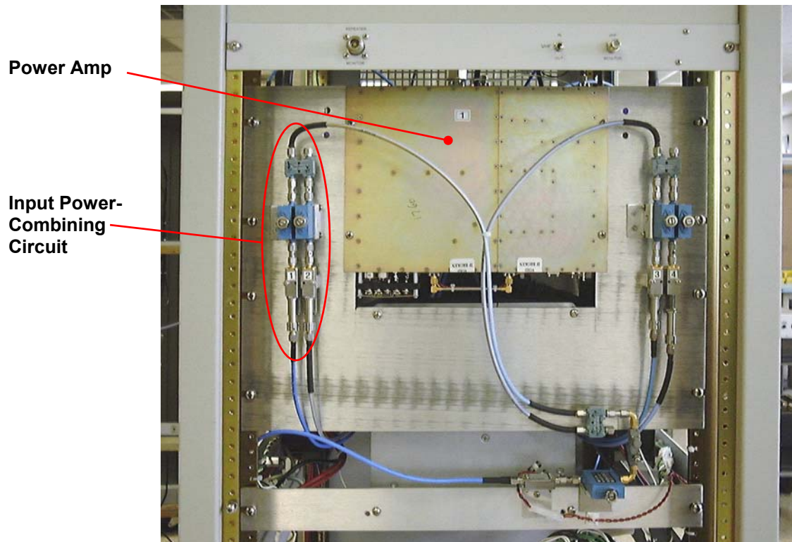
Figure 12. Front Internal View.
