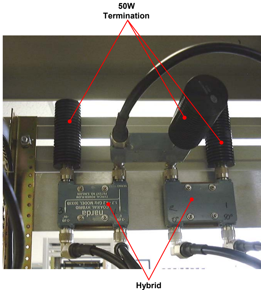
Figure 8. ITX02-2000 Internal View (right side looking up).
