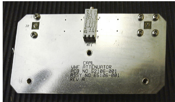
P/N: 52106-001 (Back)
